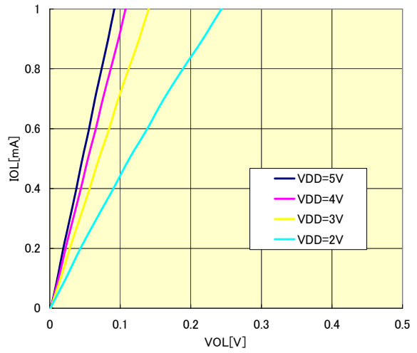
\mu PD78F0393 IOL vs VOL - VDD(P124) (Ta = 25°C)
