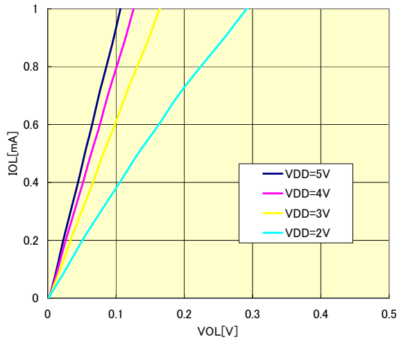
\mu PD78F0393 IOL vs VOL - VDD(P24) (Ta = 25°C)
