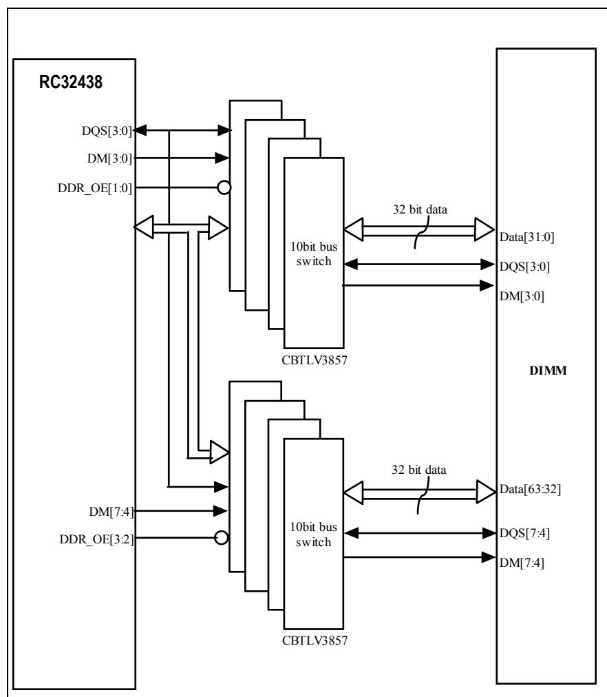
Figure 1 Data Bus Muxing for 64-bit DIMMs with RC32438 in DDR x32 Mode
