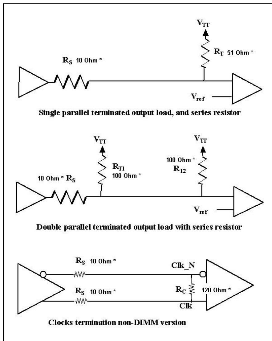
Figure 3 Termination Circuit Examples
