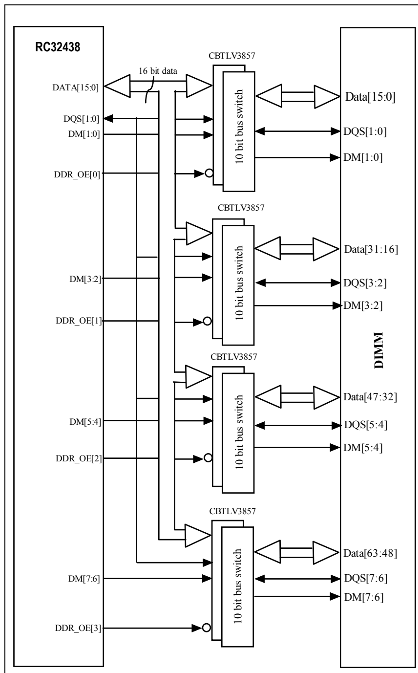
Figure 2 Data Bus Muxing for 64-bit DIMMs with RC32438 in DDR x16 Mode
