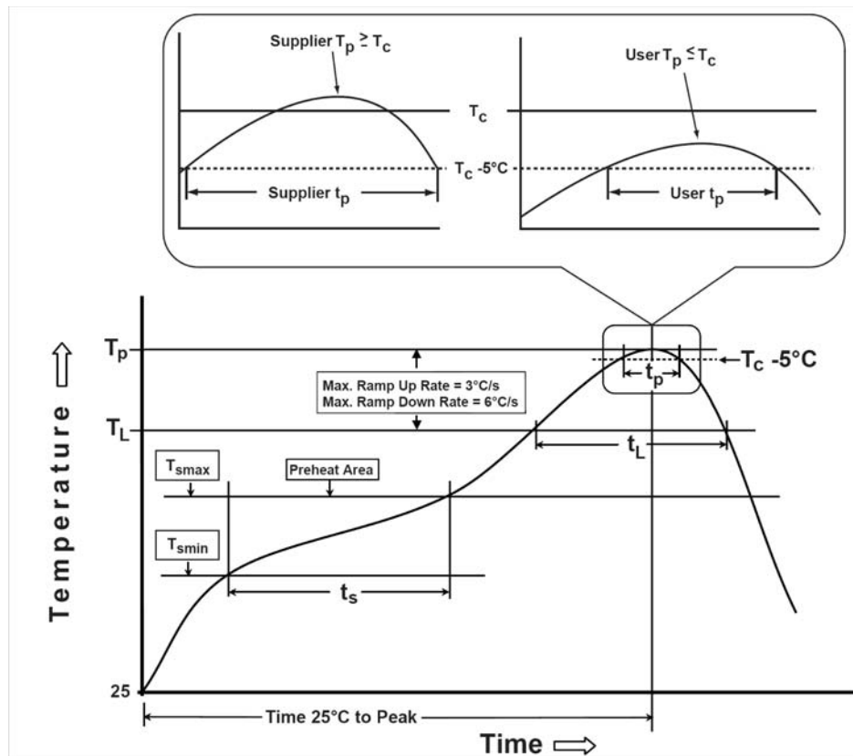
FIGURE 1. PEAK REFLOW PROFILE
