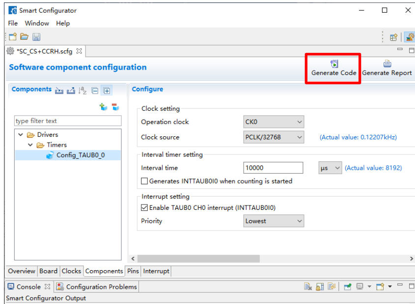
Figure 5-6. Generating code
