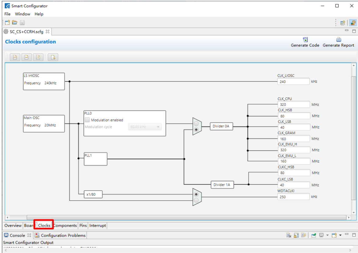
Figure 5-1. Configure clock
