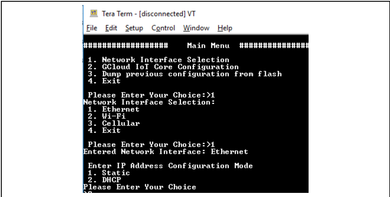
Figure 15. Ethernet Network Interface Configuration Menu
