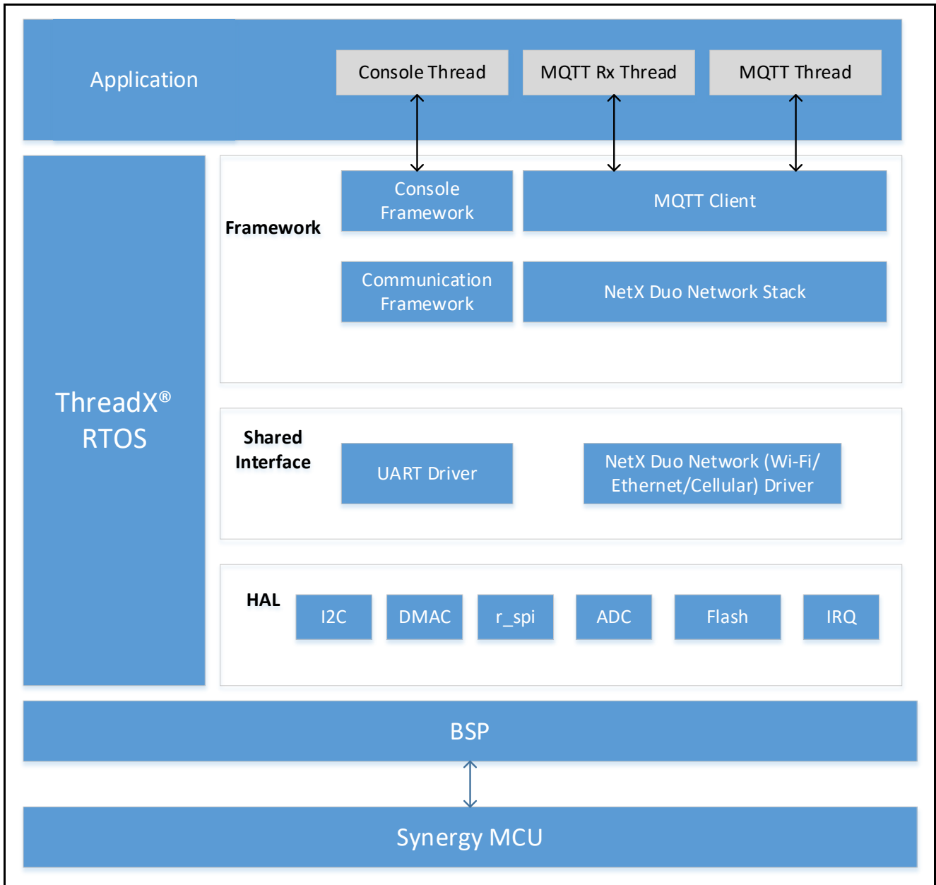
Figure 9. Synergy Cloud Connectivity Application Software Architecture
