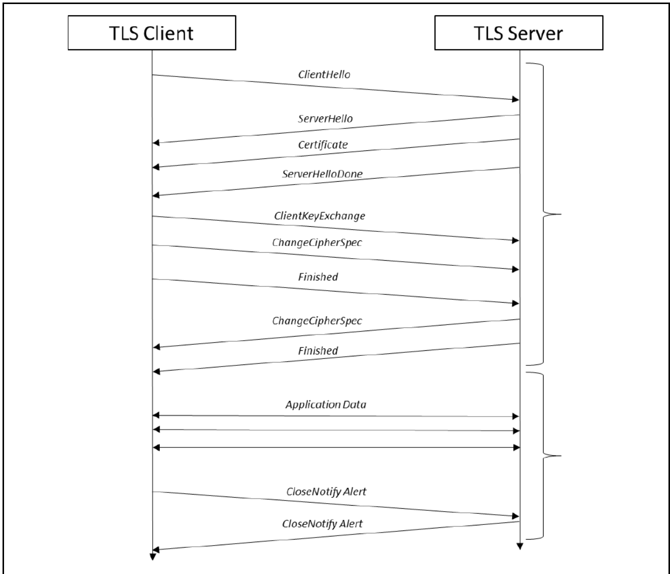
Figure 6. TLS Handshake
