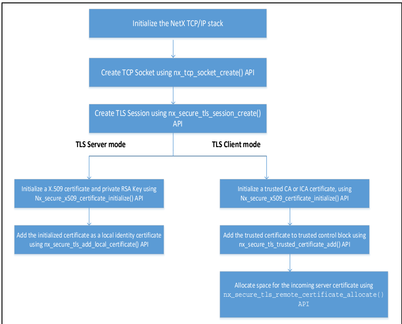
Figure 7. Synergy TLS Session Initialization
