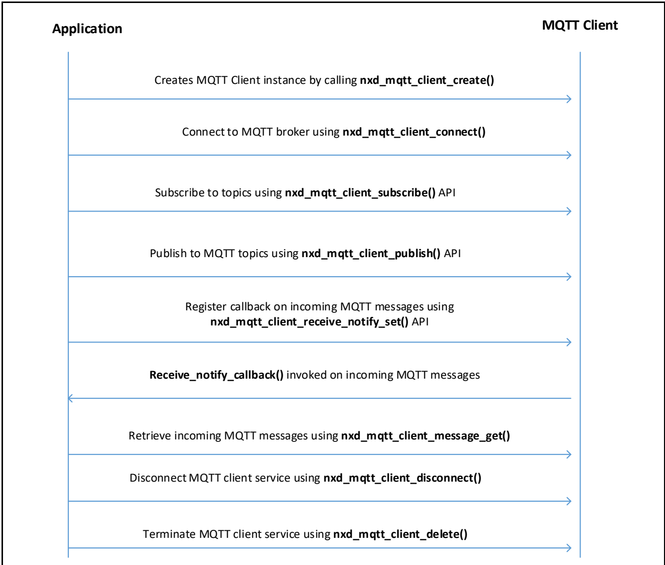
Figure 5. Synergy MQTT Client Flow Sequence
