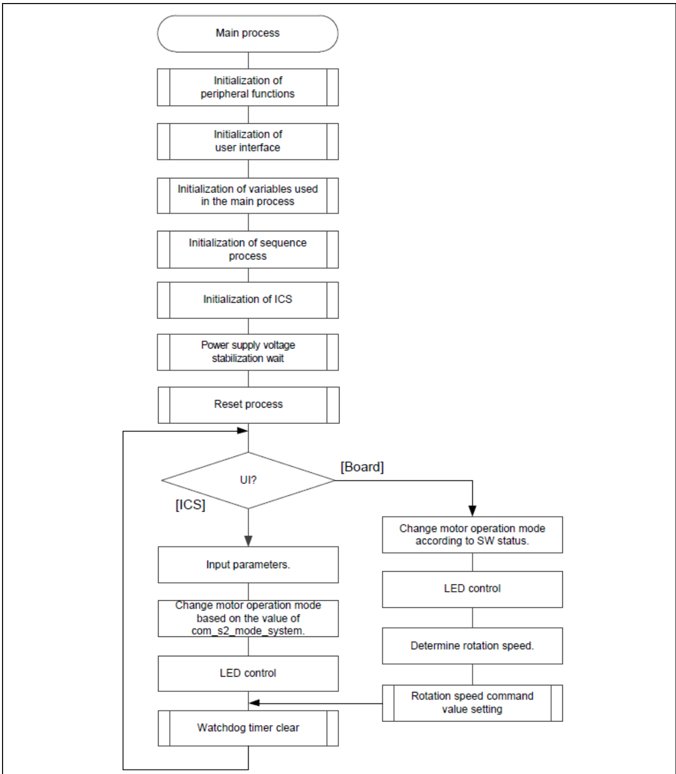
Figure 3-10 Main Process Flowchart
