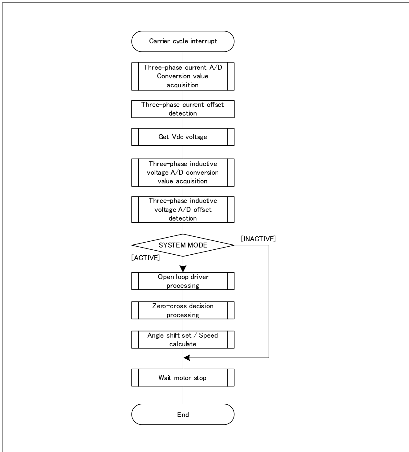
Figure 3-11 50 [μs] Periodic Interrupt Handling
