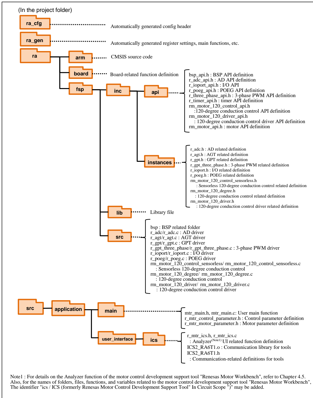
Figure 2-7 Folder and file structure
