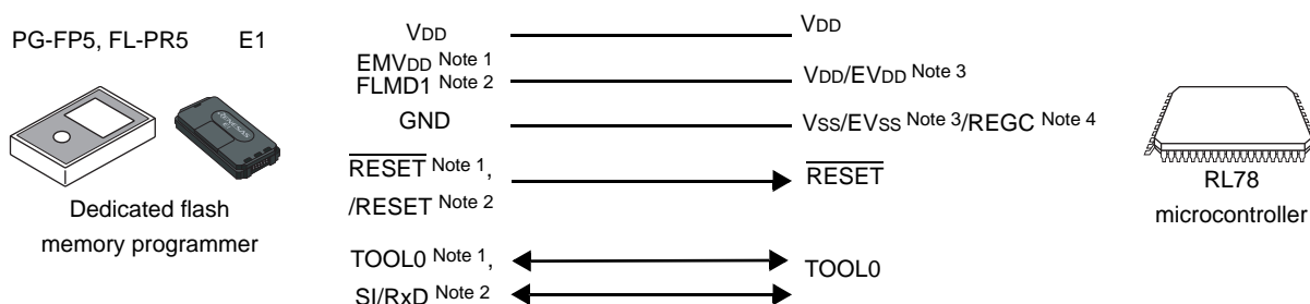
Figure 33 - 2 Communication with Dedicated Flash Memory Programmer
