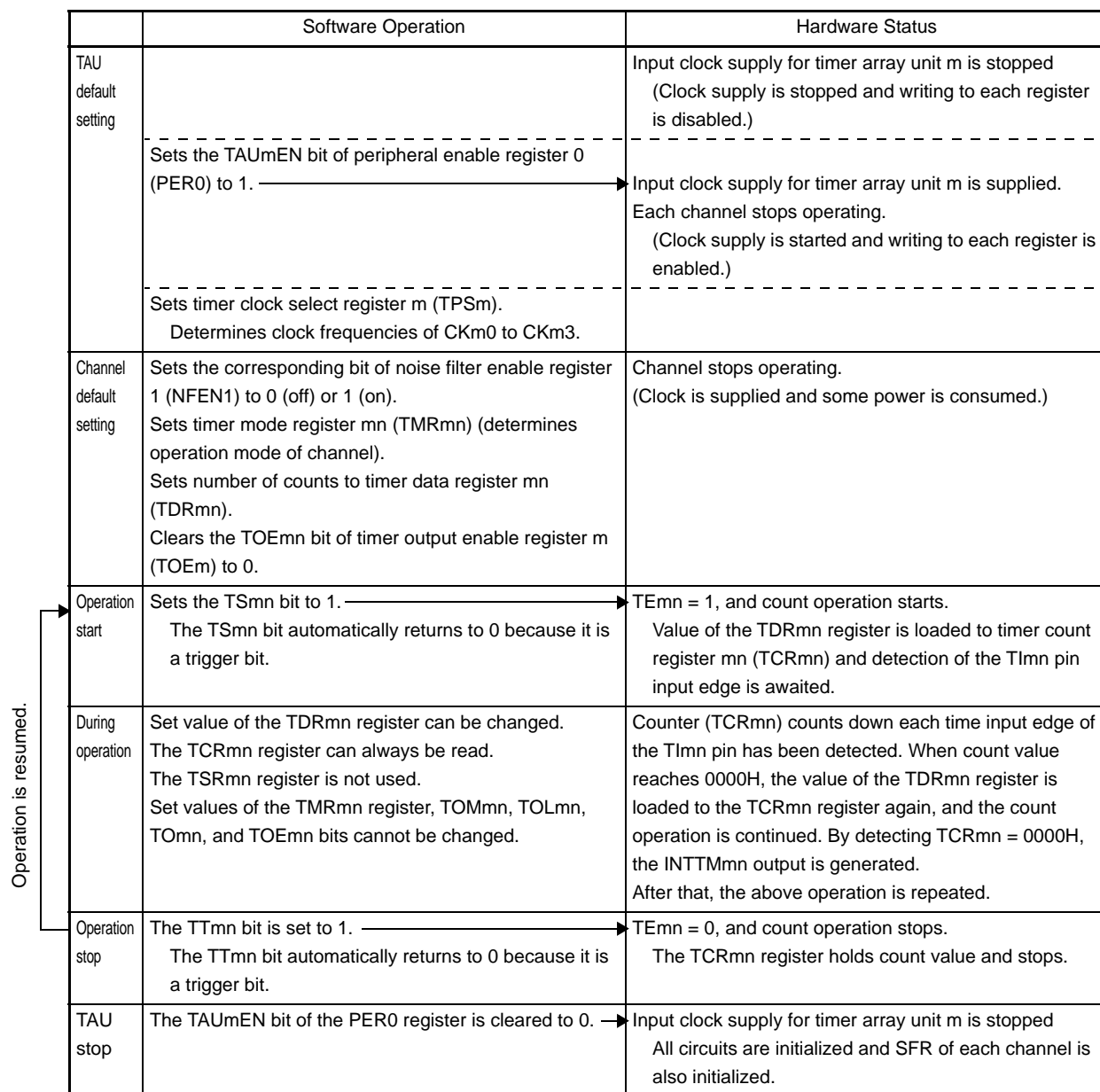
Figure 6 - 53 Operation Procedure When External Event Counter Function Is Used
