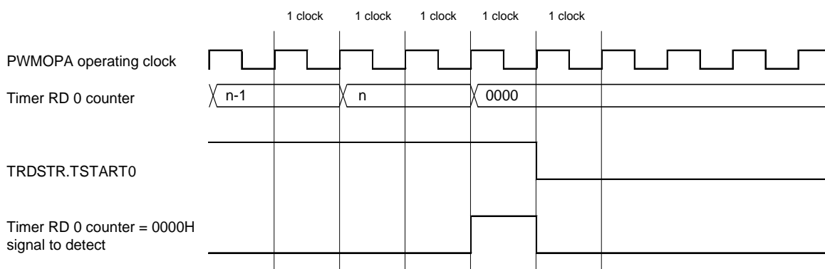
Figure 8 - 96 Judgment timing for count value = 0000H (count source = operating clock/2, count stops at the next timing after timer RD counter value becomes 0000H)
