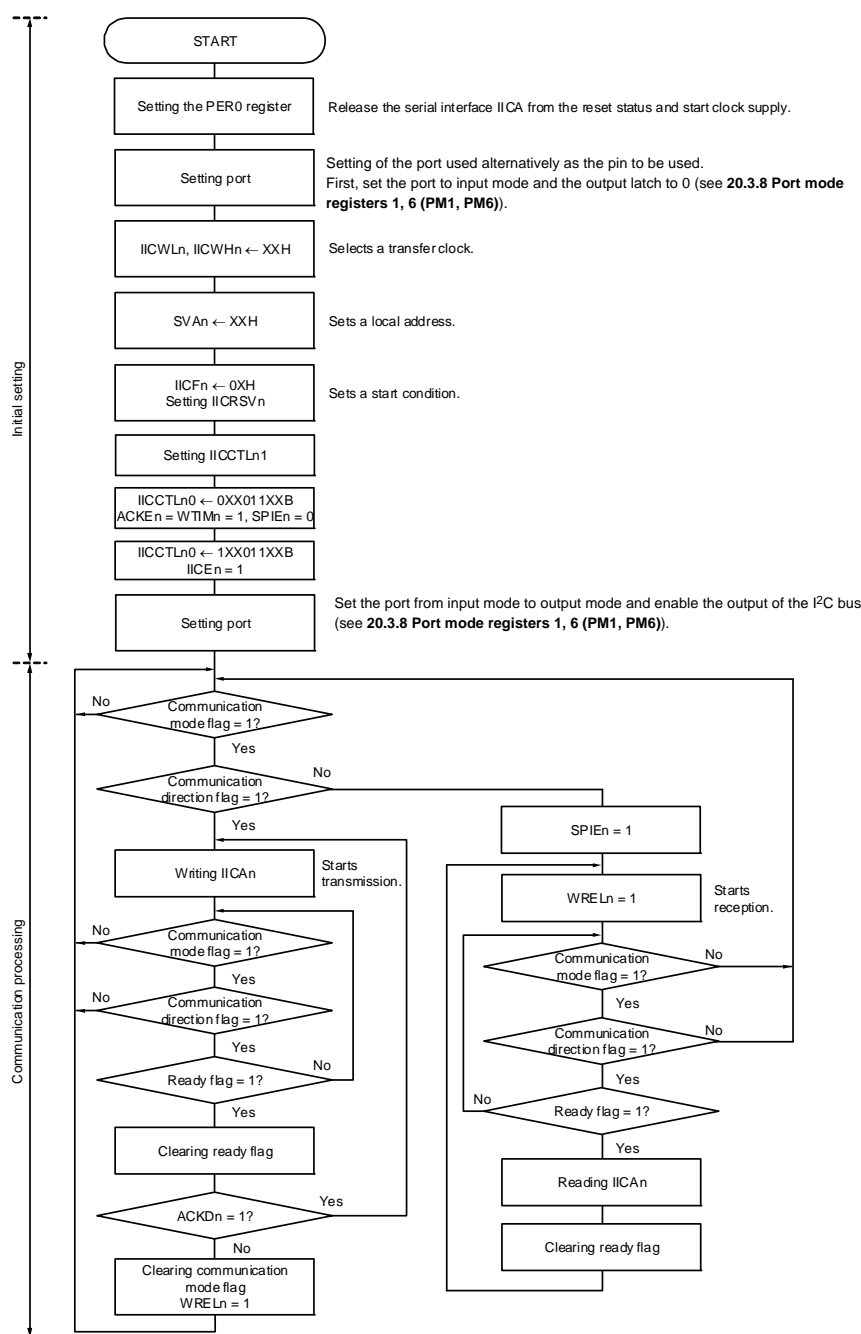
Figure 20 - 39 Slave Operation Flowchart (1)
