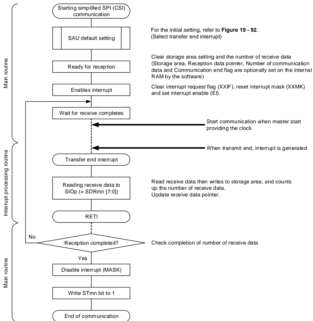
Figure 19 - 96 Flowchart of Slave Reception (in Single-Reception Mode)
