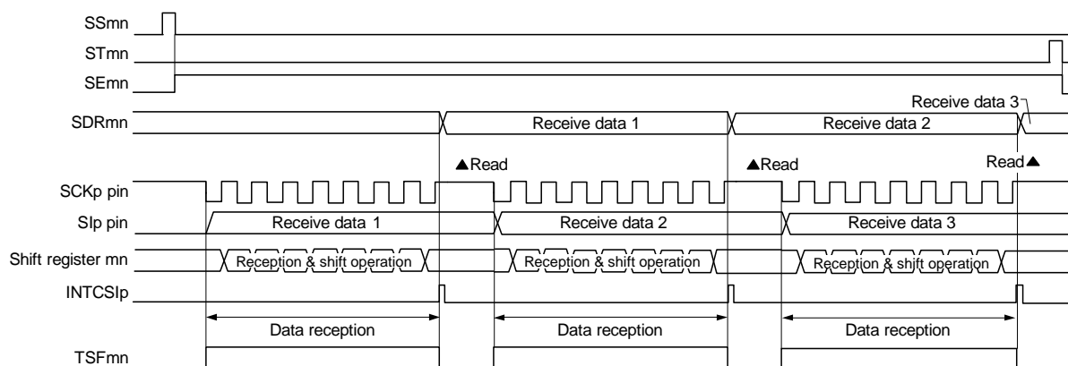
Figure 19 - 64 Timing Chart of Slave Reception (in Single-Reception Mode)
