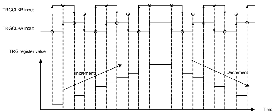
Figure 9 - 28 Operation Example 2 in Phase Counting Mode
