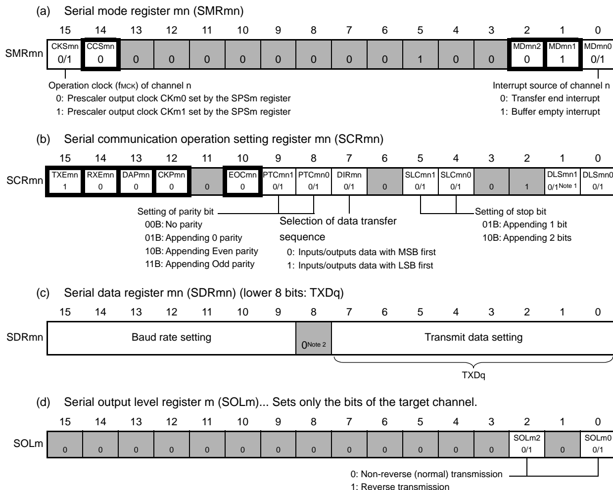
Figure 19 - 107 Example of Contents of Registers for UART Transmission of UART (UART0 to UART2) (1/2)
