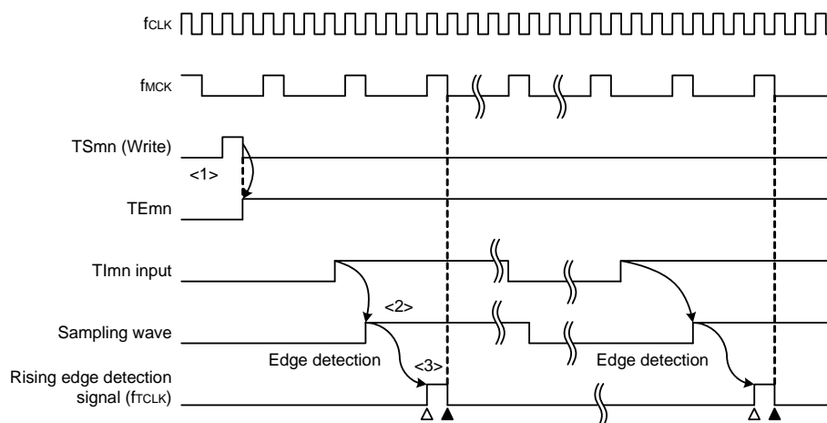
Figure 6 - 28 Timing of f CLK and Count Clock (f TCLK ) (When CCSmn = 1, noise filter unused)
