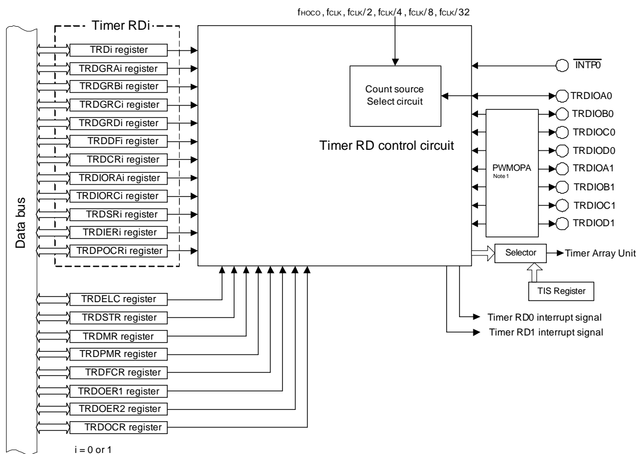
Figure 8 - 1 Timer RD Block Diagram
