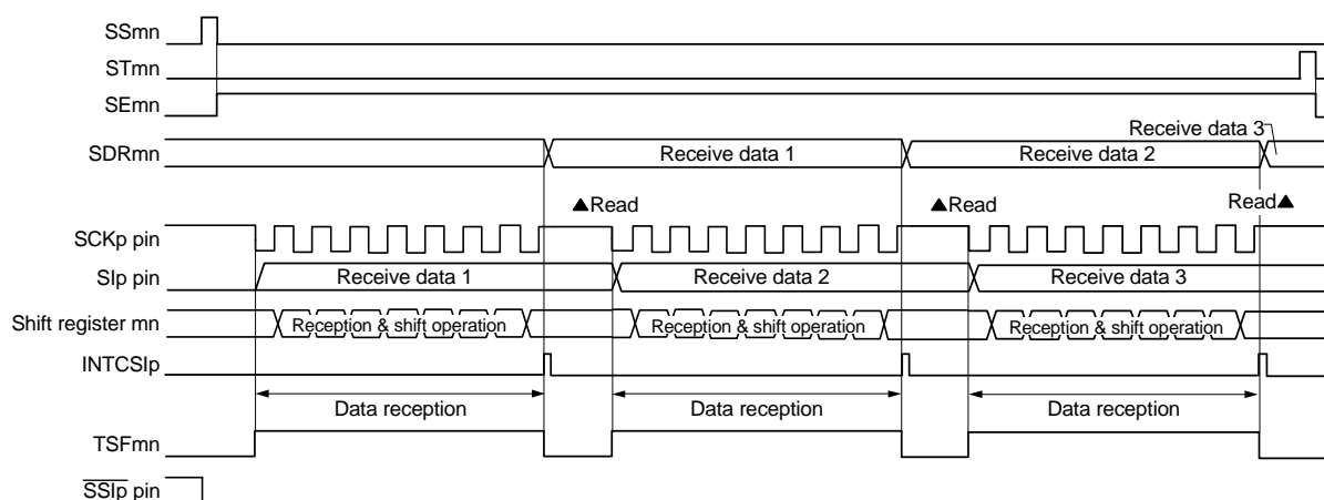
Figure 19 - 95 Timing Chart of Slave Reception (in Single-Reception Mode) (Type 1: DAPmn = 0, CKPmn = 0)
