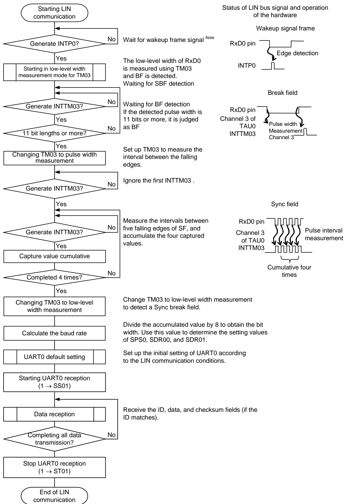
Figure 19 - 134 Flowchart for LIN Reception
