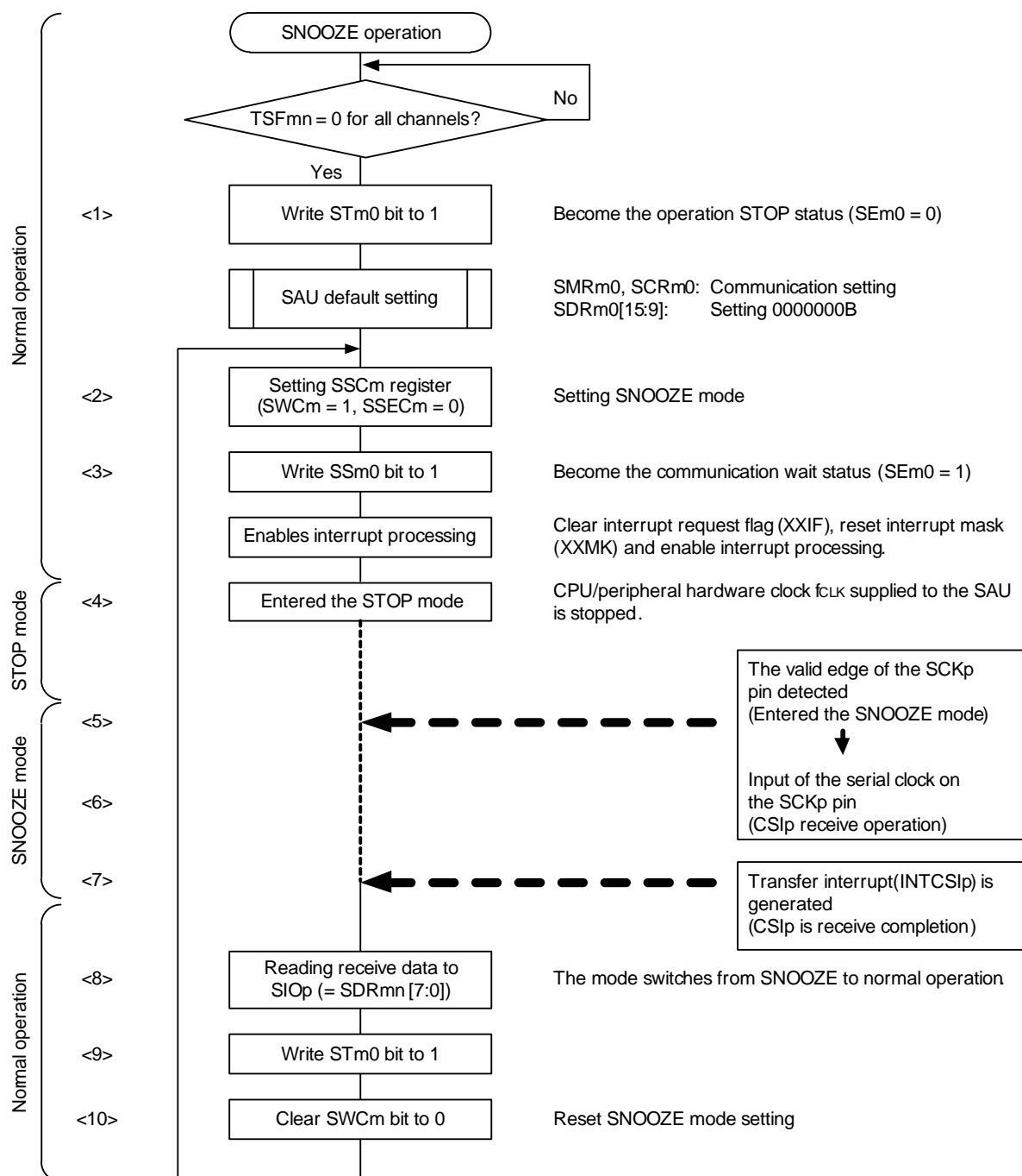
Figure 19 - 77 Flowchart of SNOOZE Mode Operation (continuous startup)
