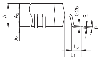
Detail F
