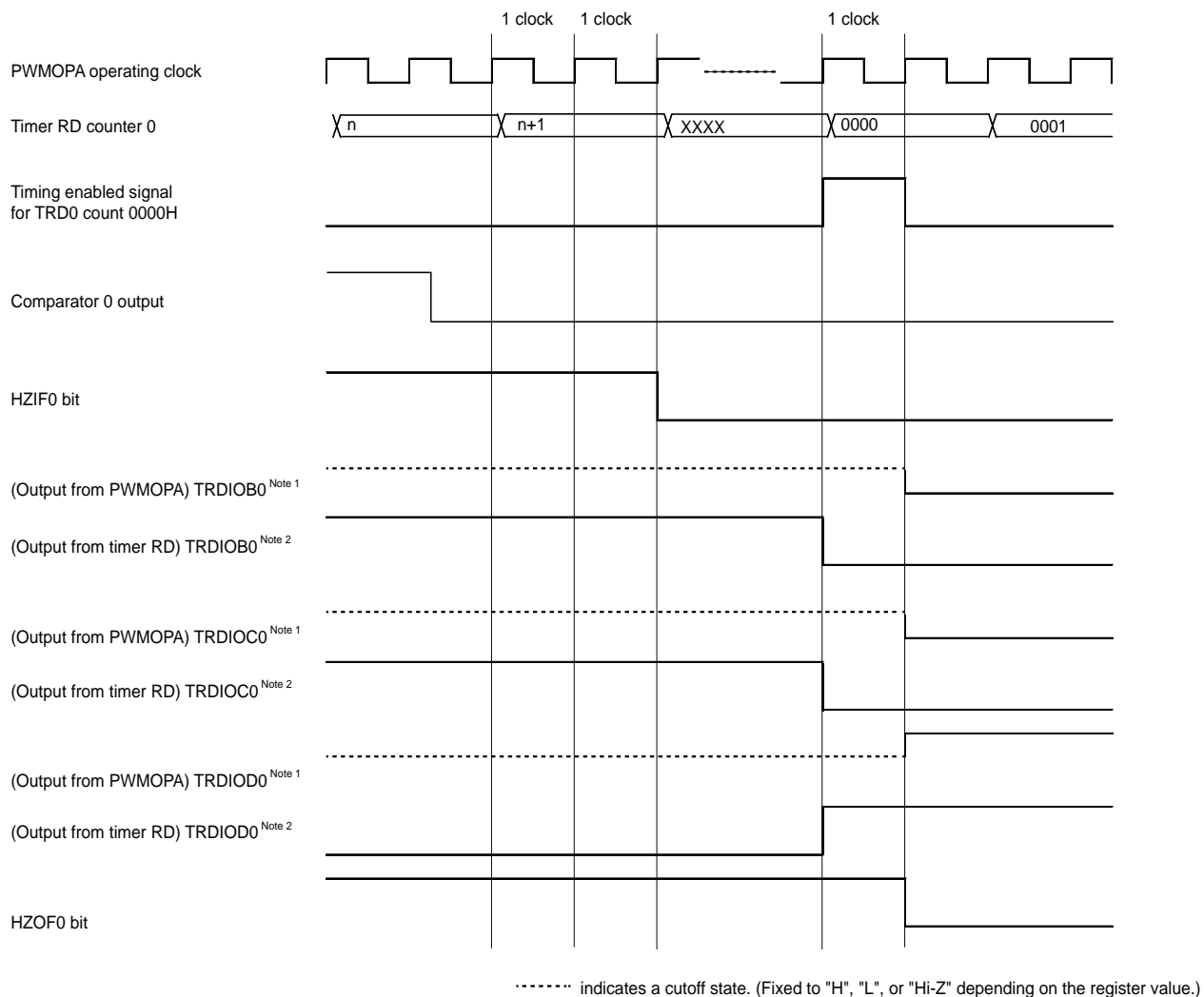
Figure 8 - 78 Cutoff release detailed timing diagram (timer RD count source = f CLK /2)
