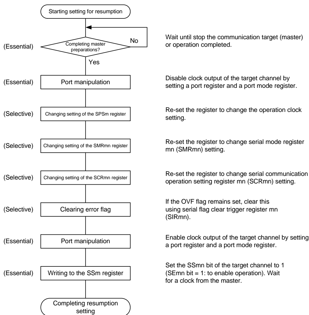
Figure 19 - 63 Procedure for Resuming Slave Reception
