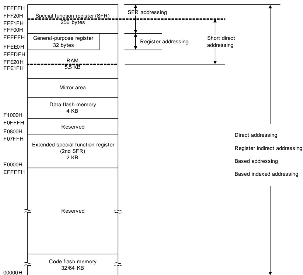
Figure 3 - 4 Correspondence Between Data Memory and Addressing
