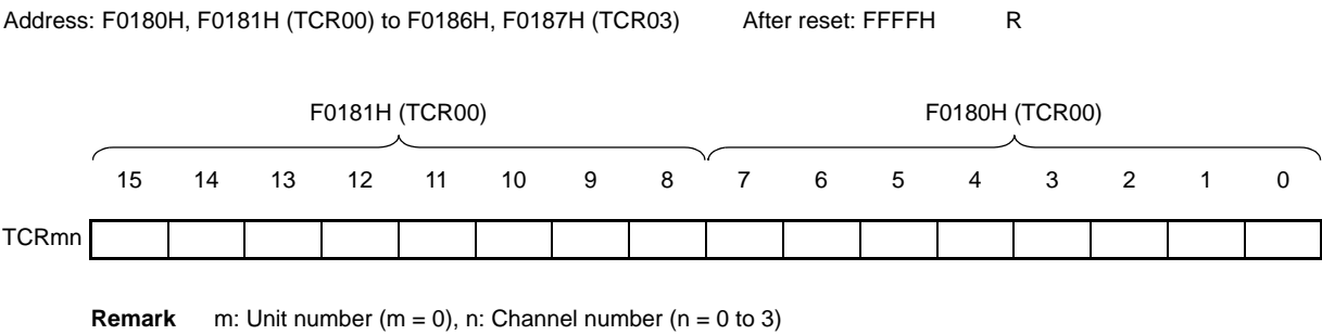
Figure 6 - 6 Format of Timer count register mn (TCRmn)
