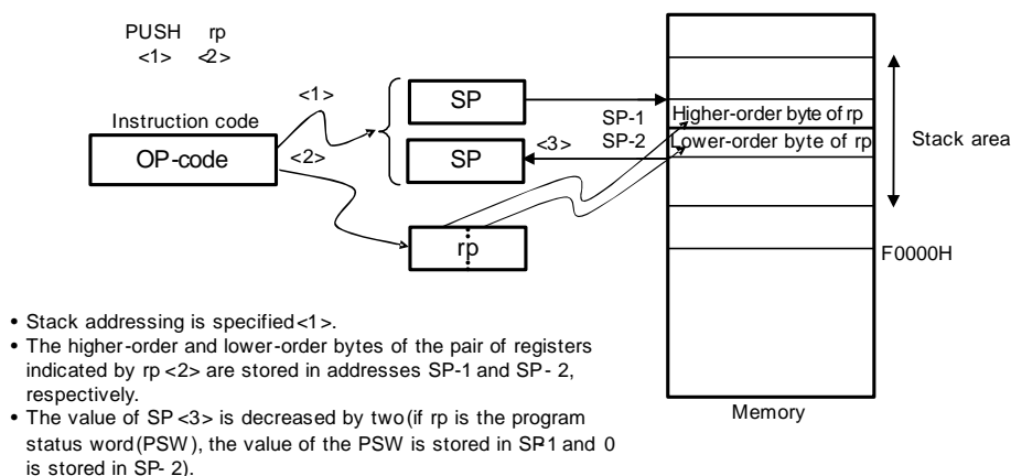
Figure 3 - 33 Example of PUSH rp
