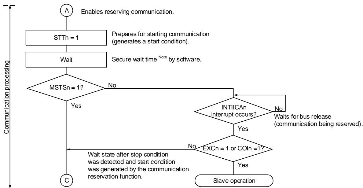
Figure 20 - 37 Master Operation in Multi-Master System (2/3)
