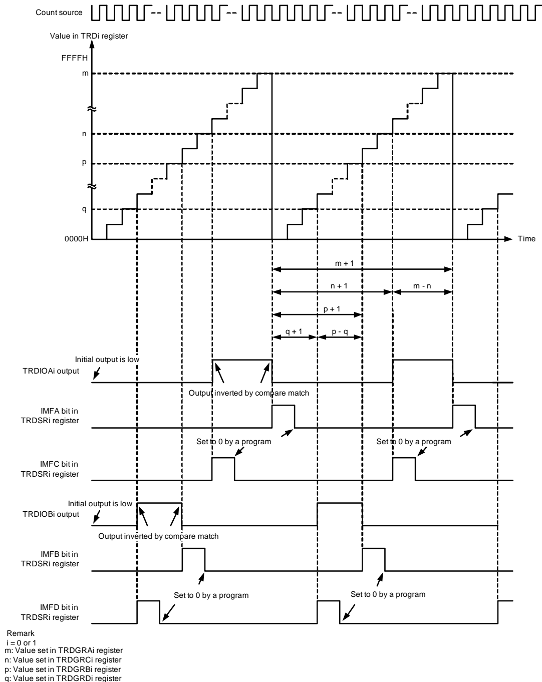
Figure 8 - 53 Operation Example When TRDGRCi Register is Used for Output Control of TRDIOAi Pin and TRDGRDi Register is Used for Output Control of TRDIOBi Pin
