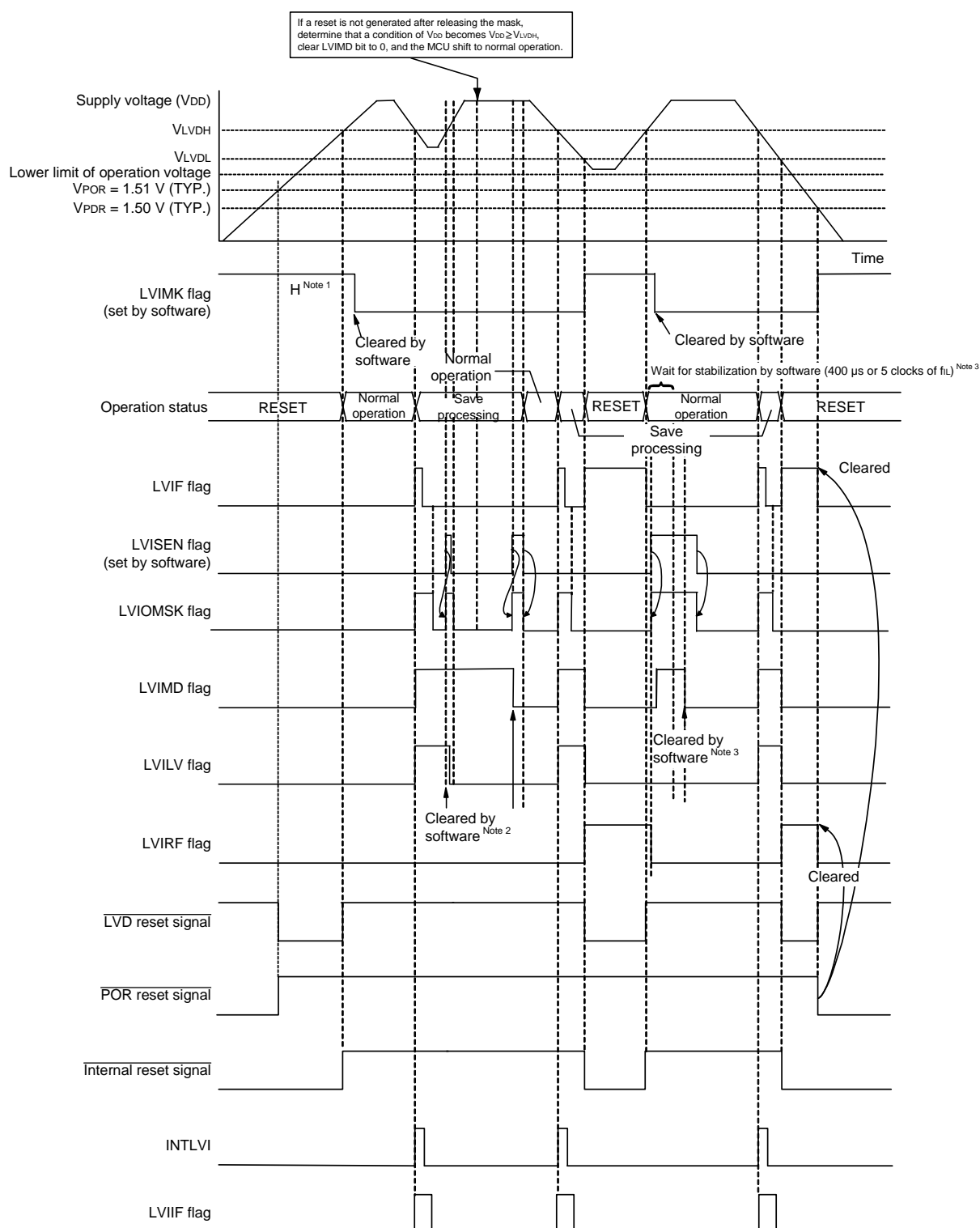
Figure 29 - 8 Timing of Voltage Detector Reset Signal and Interrupt Signal Generation (Option Byte LVIMDS1, LVIMDS0 = 1, 0) (1/2)
