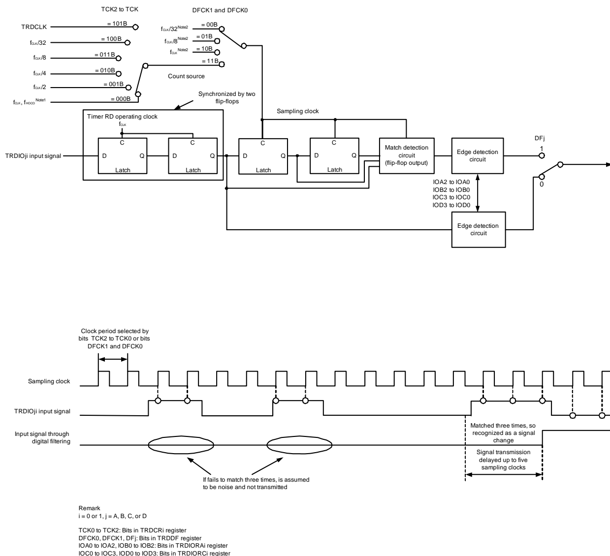
Figure 8 - 49 Block Diagram of Digital Filter
