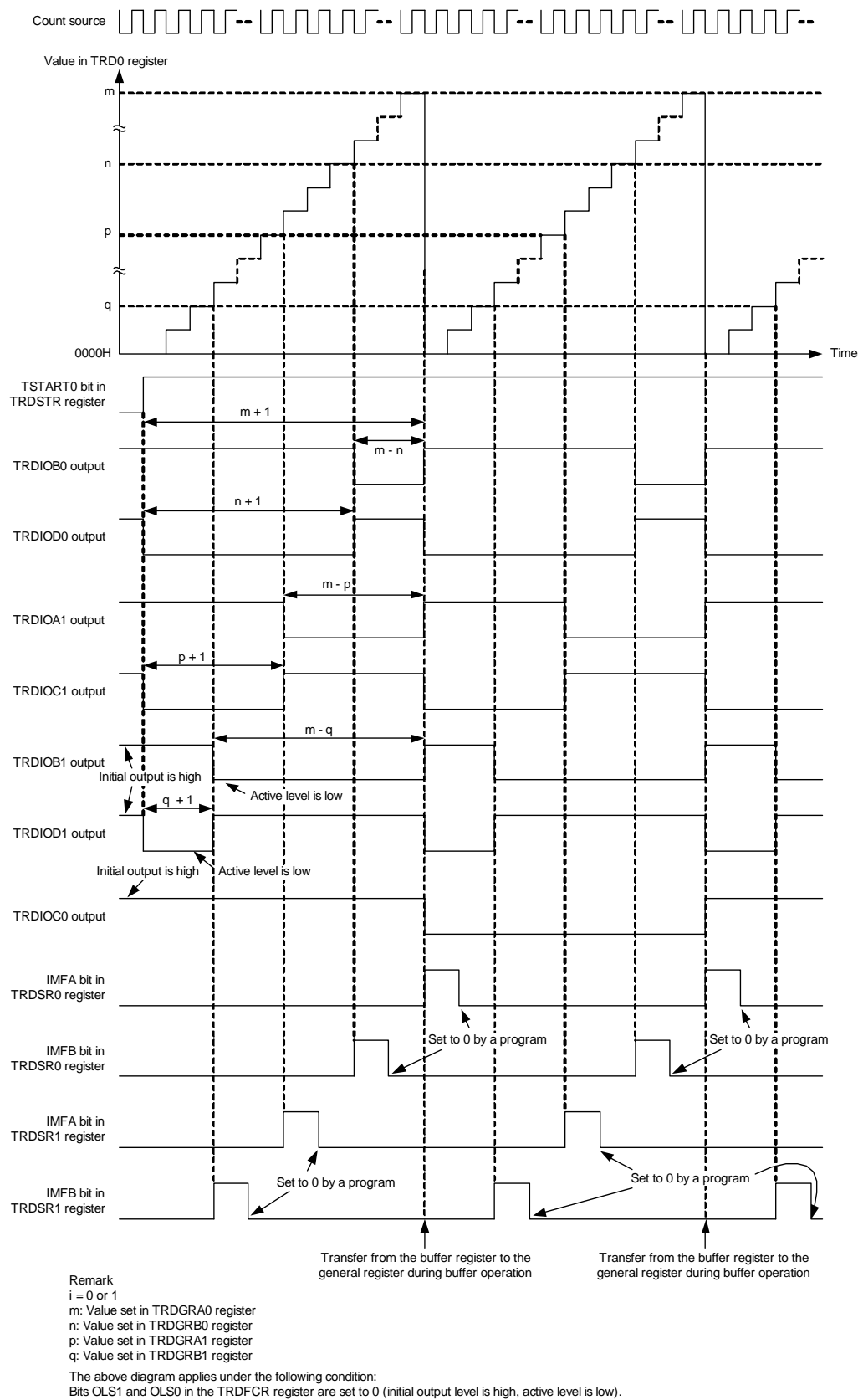
Figure 8 - 58 Operation Example in Reset Synchronous PWM Mode
