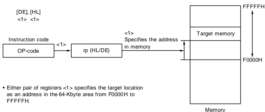
Figure 3 - 22 Example of [DE], [HL]
