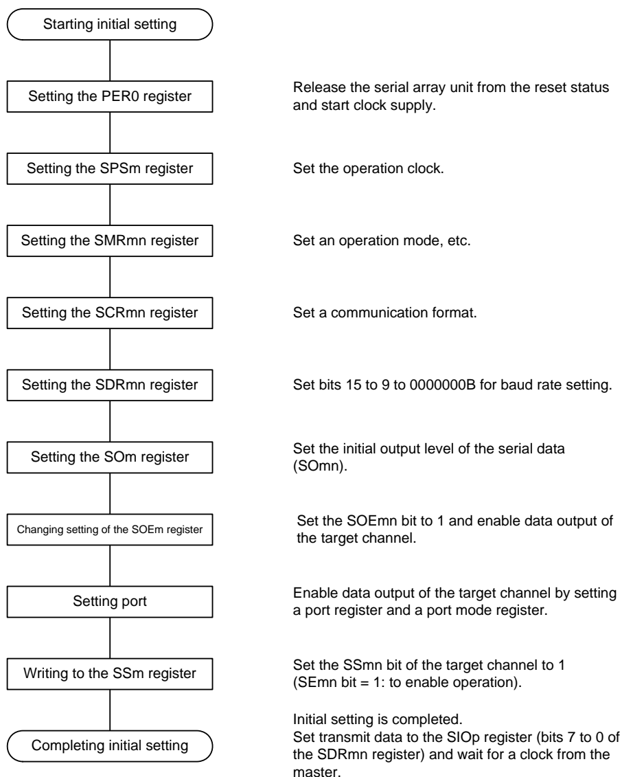
Figure 19 - 53 Initial Setting Procedure for Slave Transmission
