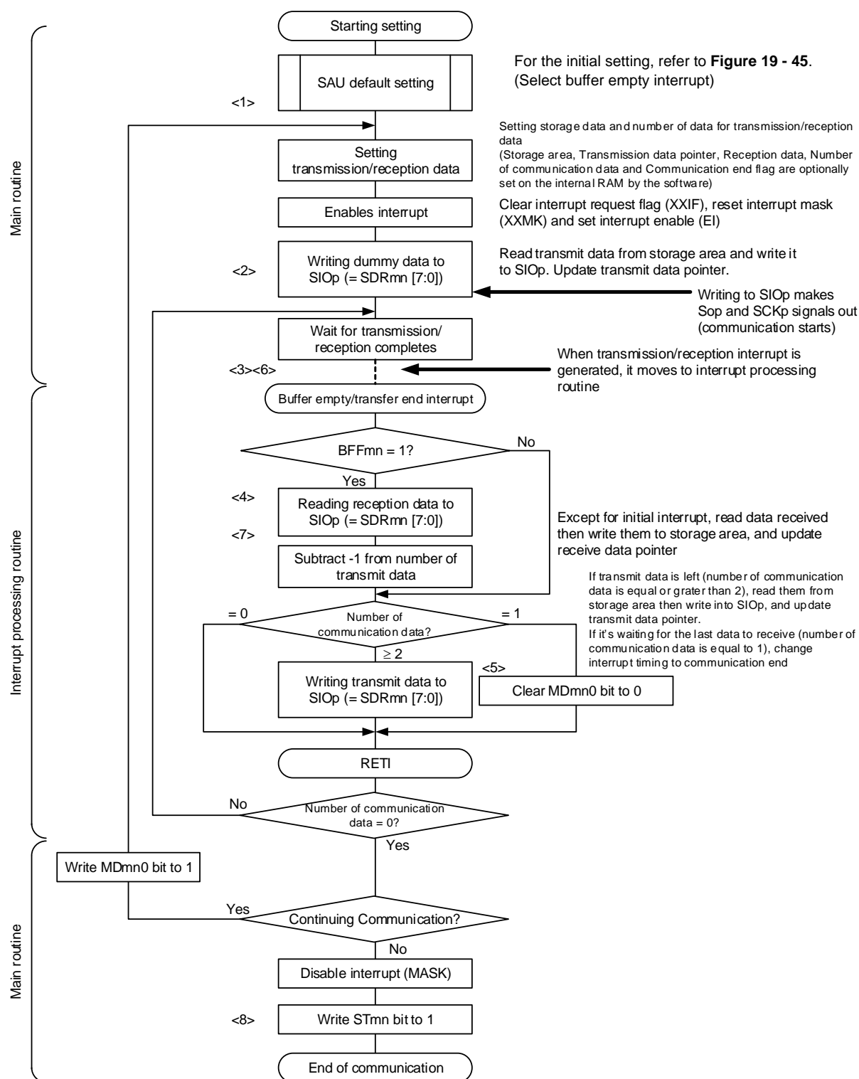
Figure 19 - 51 Flowchart of Master Transmission/Reception (in Continuous Transmission/Reception Mode)
