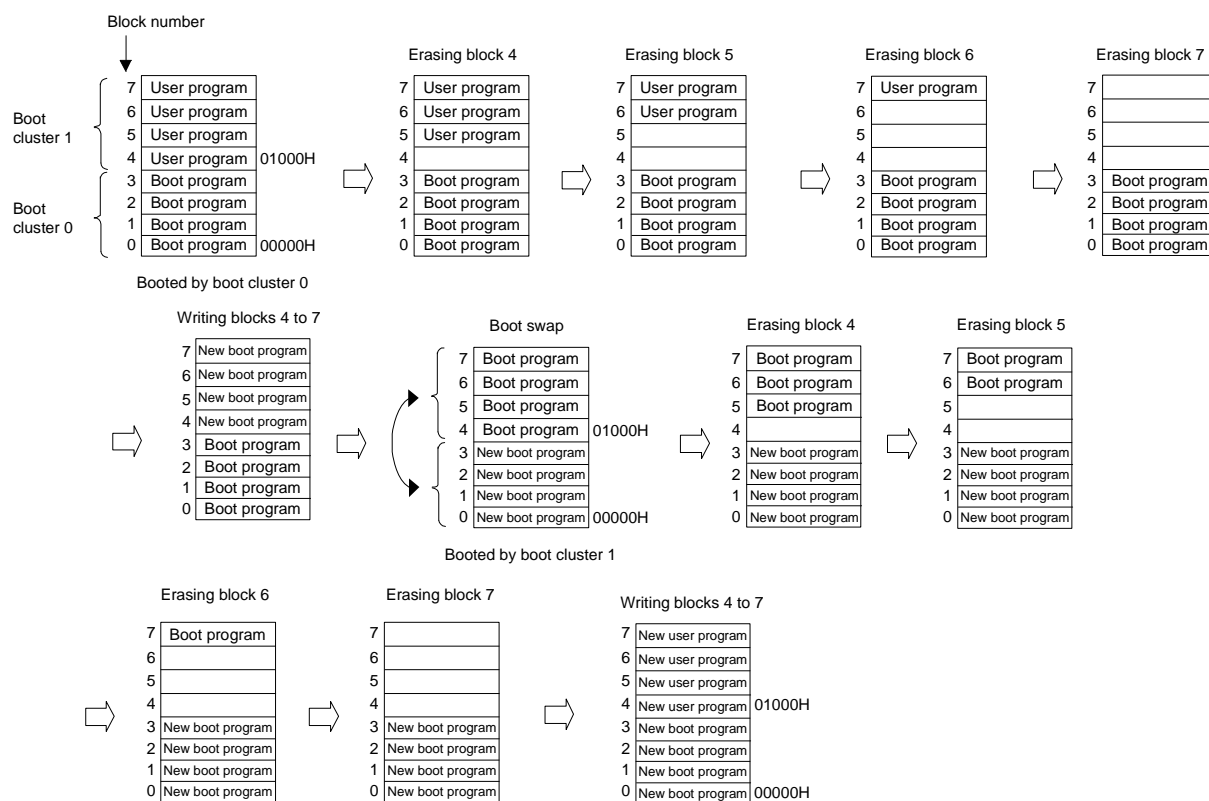
Figure 33 - 10 Example of Executing Boot Swapping
