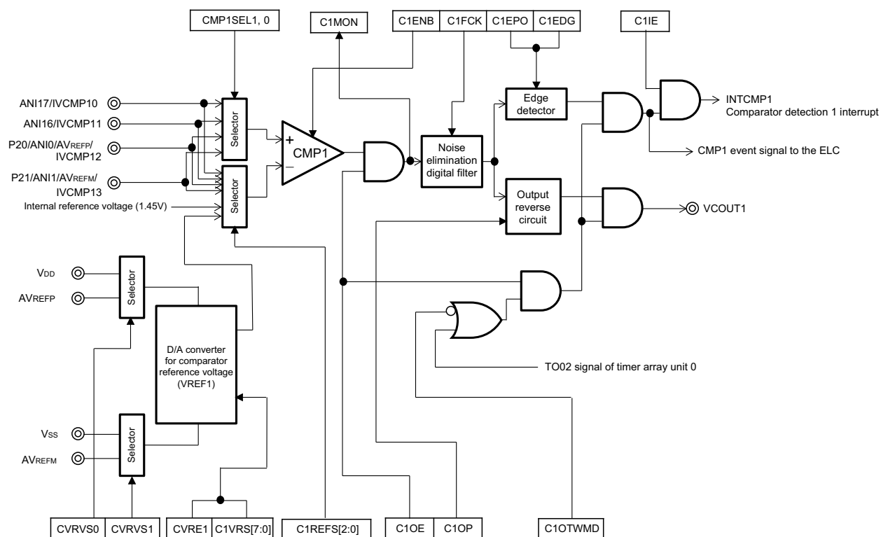
Figure 17 - 2 Comparator 1 Block Diagram
