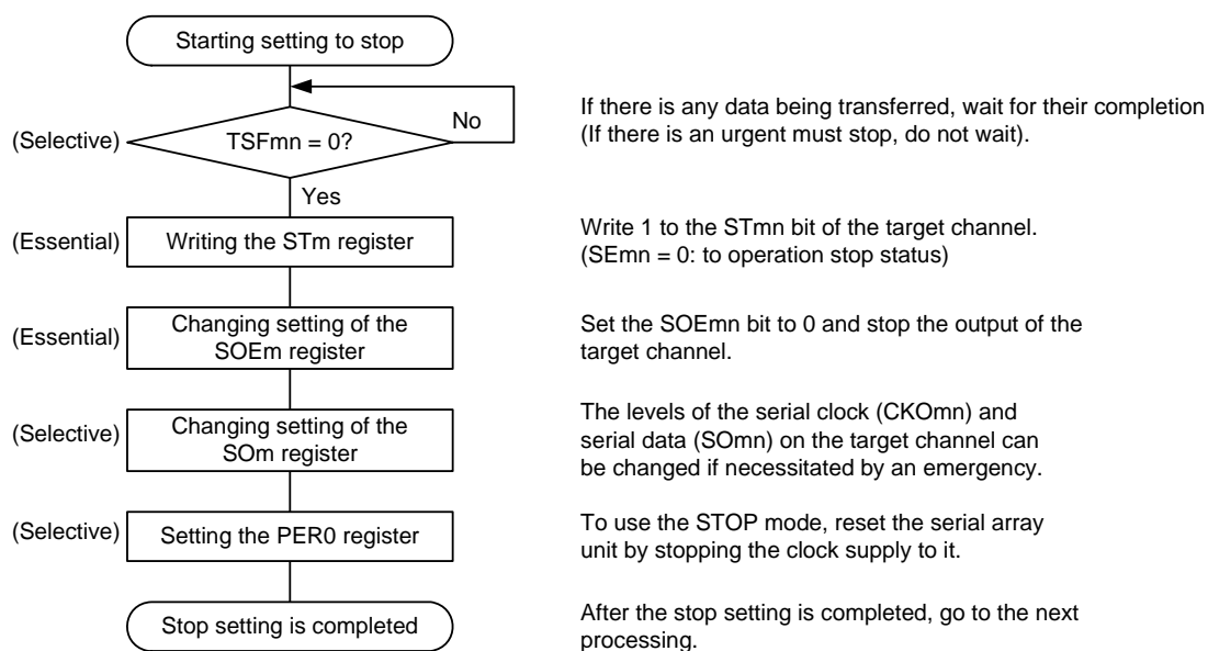
Figure 19 - 30 Procedure for Stopping Master Transmission
