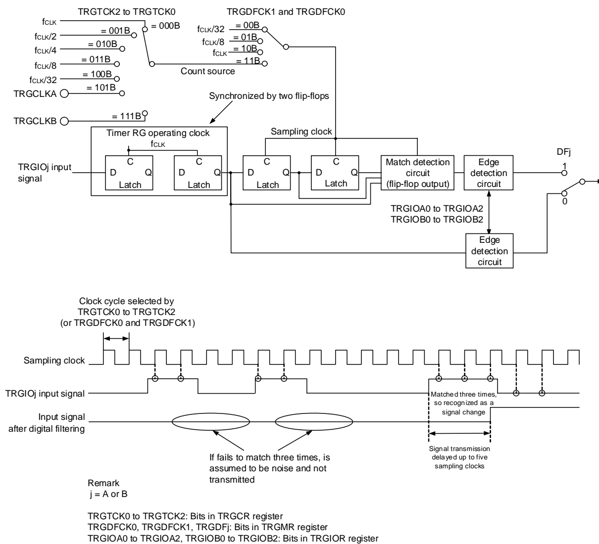
Figure 9 - 15 Block Diagram of Digital Filter
