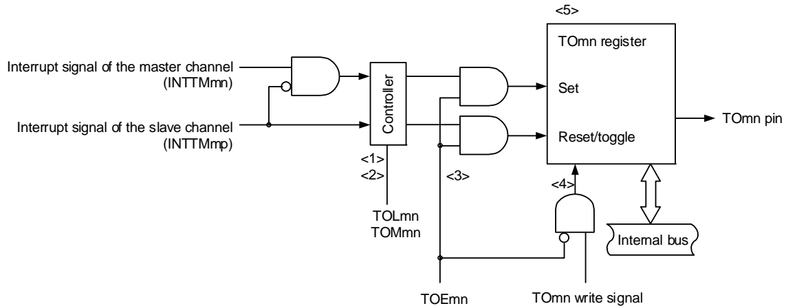
Figure 6 - 34 Output Circuit Configuration
