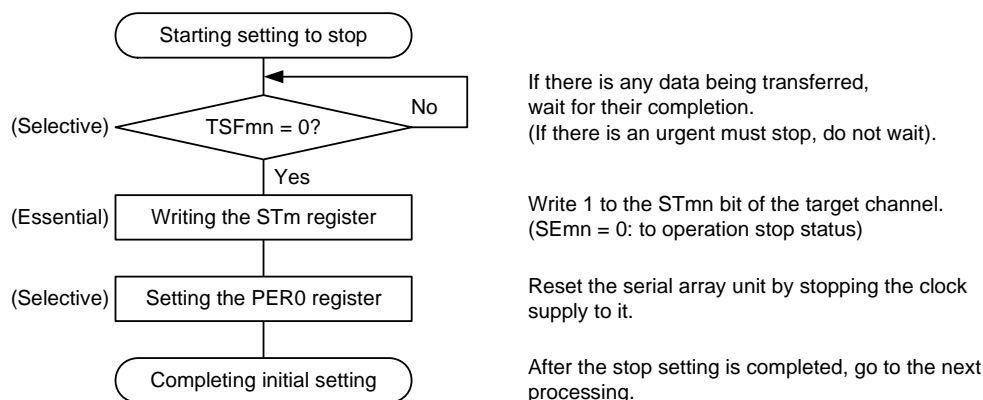
Figure 19 - 119 Procedure for Stopping UART Reception
