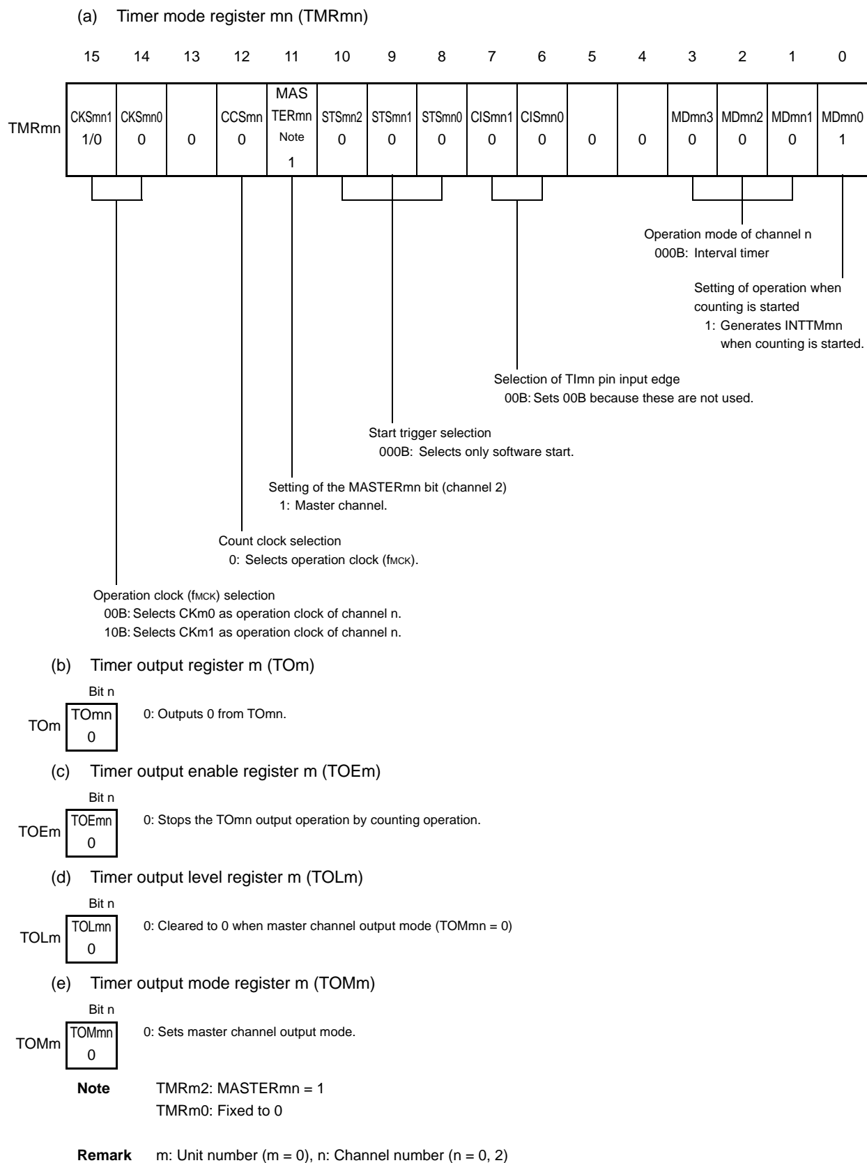
Figure 6 - 78 Example of Set Contents of Registers When PWM Function (Master Channel) Is Used
