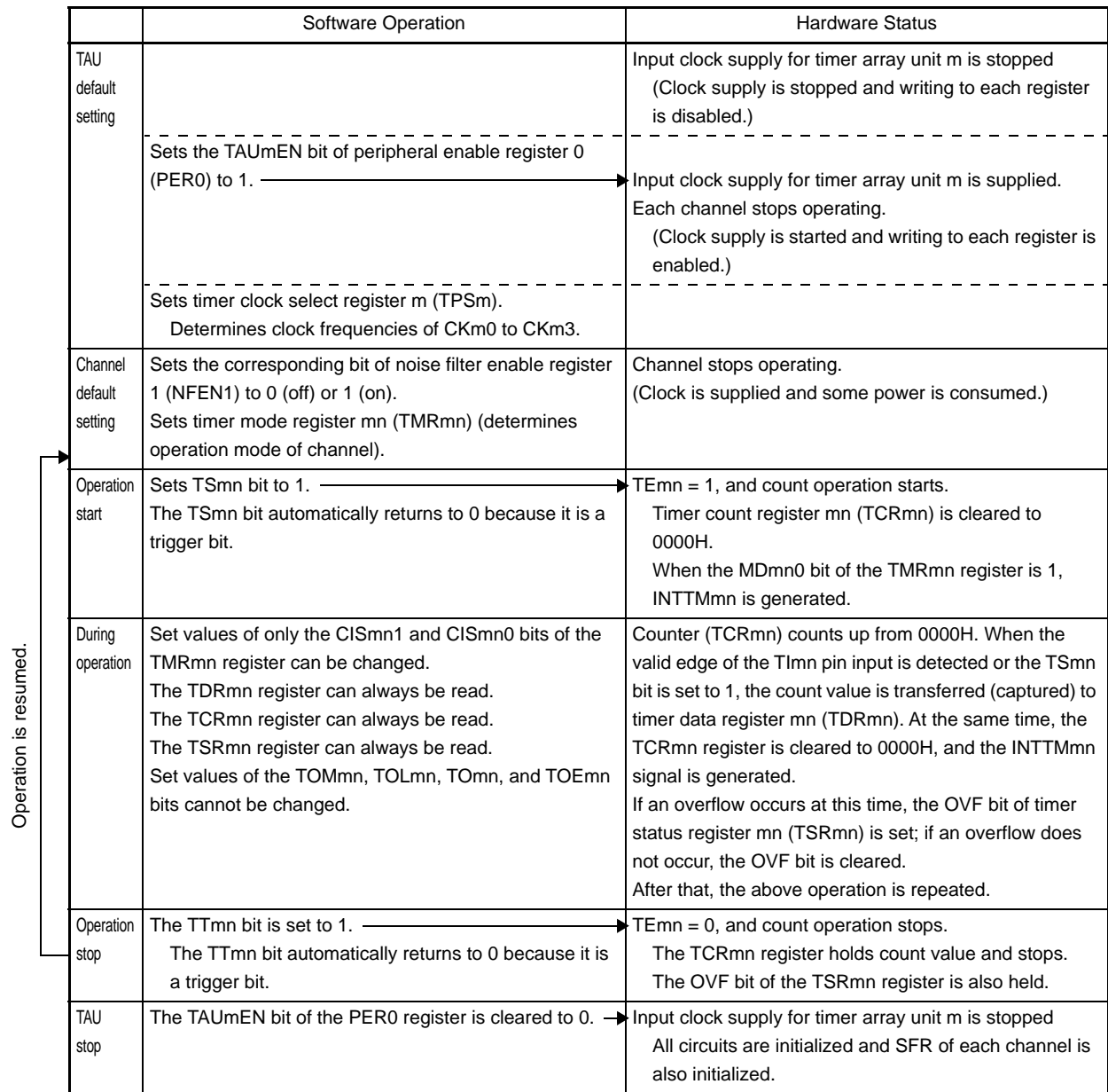
Figure 6 - 61 Operation Procedure When Input Pulse Interval Measurement Function Is Used
