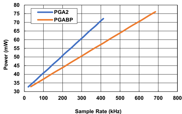
Figure 83. Power vs Sample Rate
