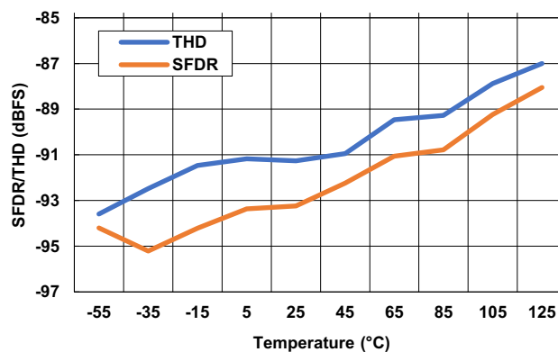
Figure 76. SFDR and THD vs Temperature
