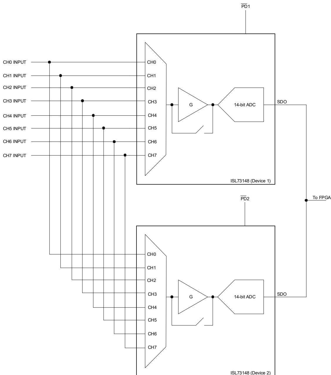
Figure 126. ISL73148SEH Cold Sparing Example Circuit
