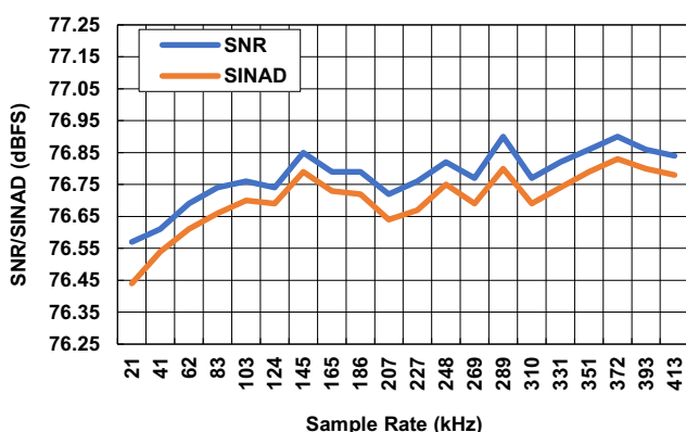
Figure 79. SNR and SINAD vs Sample Rate
