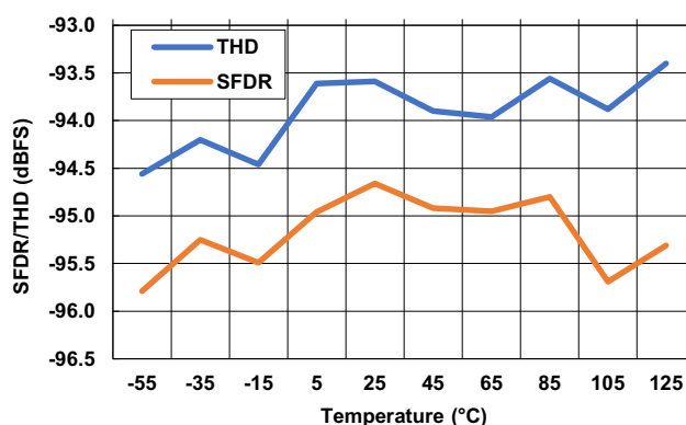
Figure 34. SFDR and THD vs Temperature - PGA Bypassed
