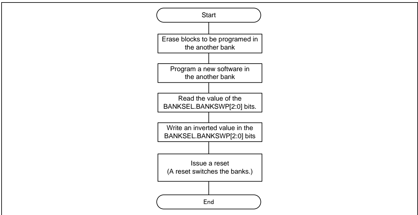
Figure 2.13 Flow for Switching the Start-Up Bank
