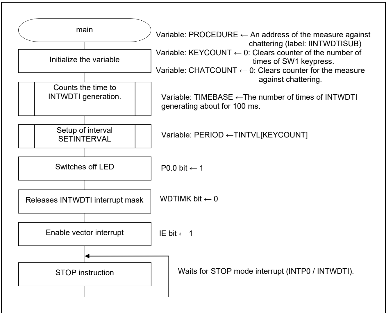
Figure 5.7 Main Processing
