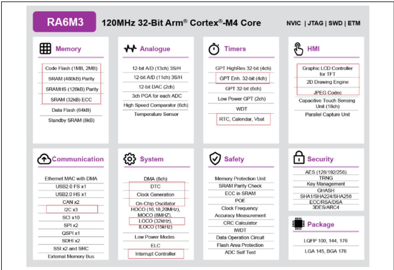
Figure 4. RA6M3 MCU Peripherals Used in the Graphics Application
