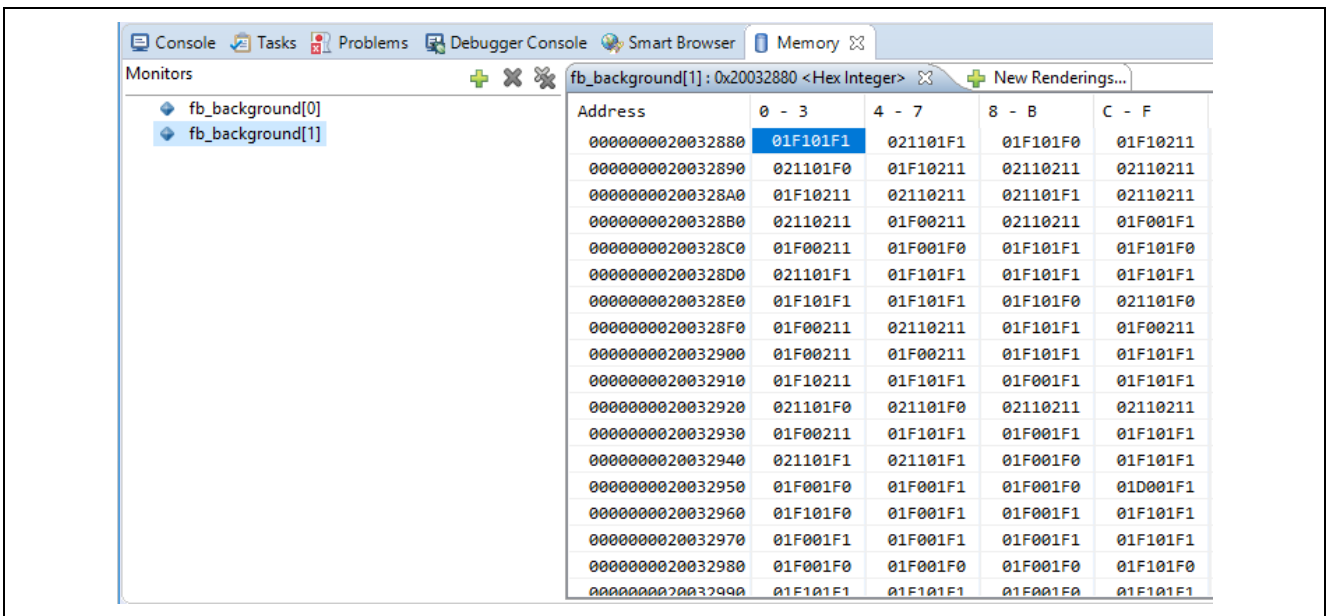
Figure 56. Framebuffer 1 Contents
