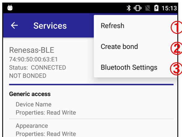
Figure 6-16 Overflow Menu.
