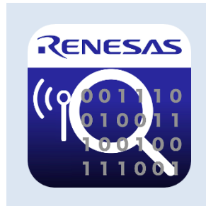
Figure 5-1 GATTBrowser icon.
