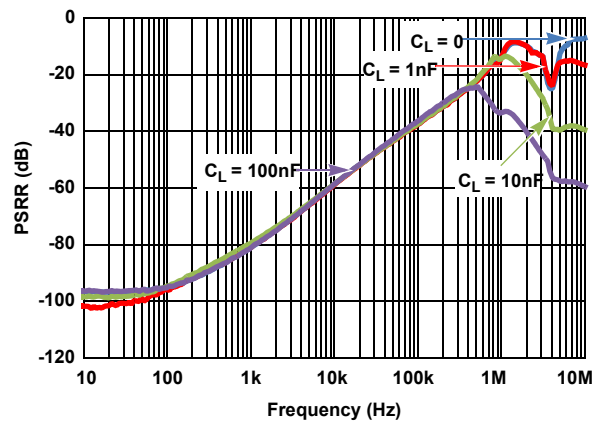
Figure 20. PSRR at Different Capacitive Loads
