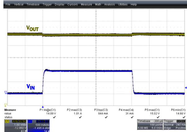
FIGURE 18. V_{IN} = 30V , V_{OUT} = 15V , I_{OUT} 0 -1A STEP
