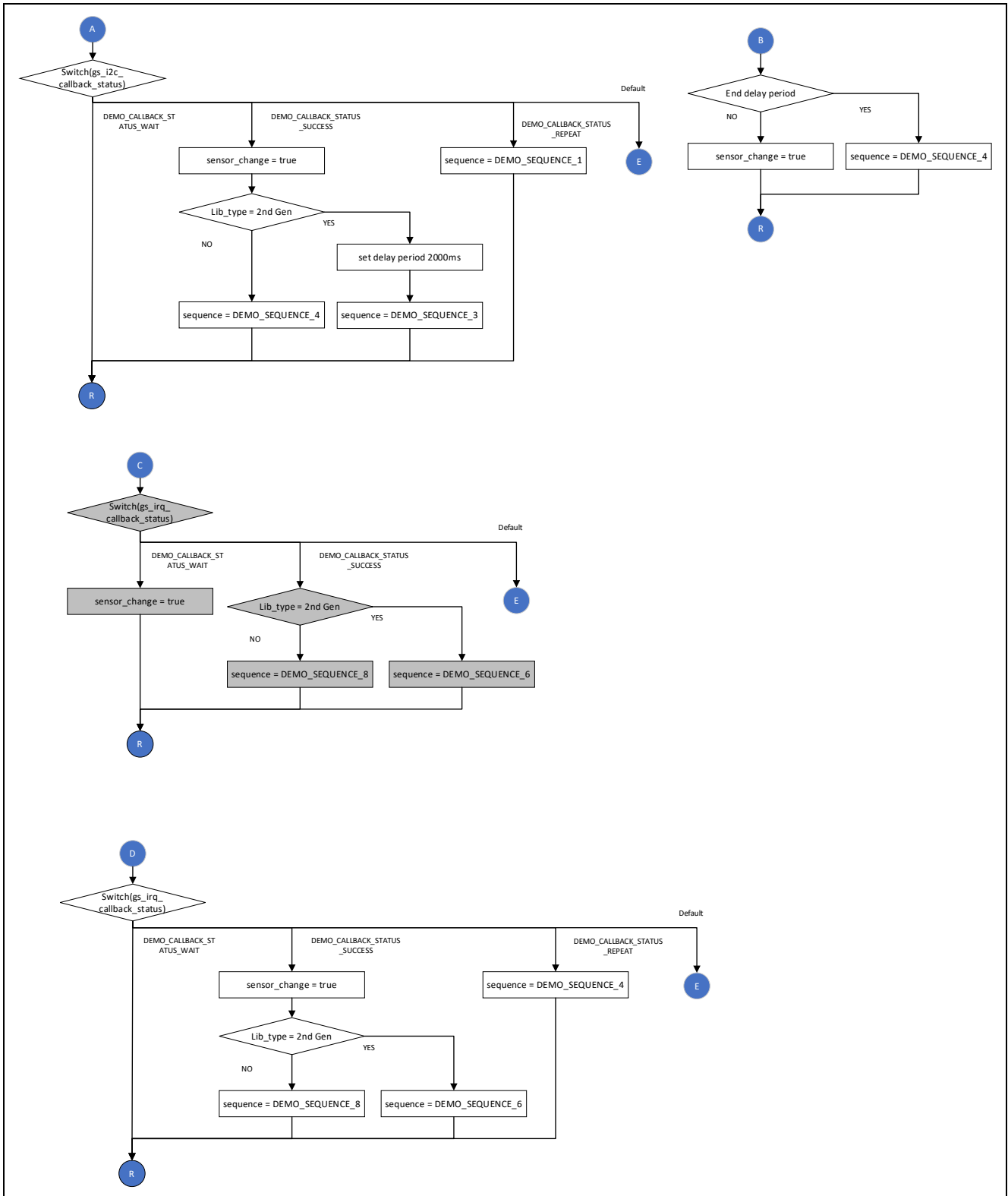
Figure 6-7 Flow 2 of ZMOD4510 Sample Software Main Processing
