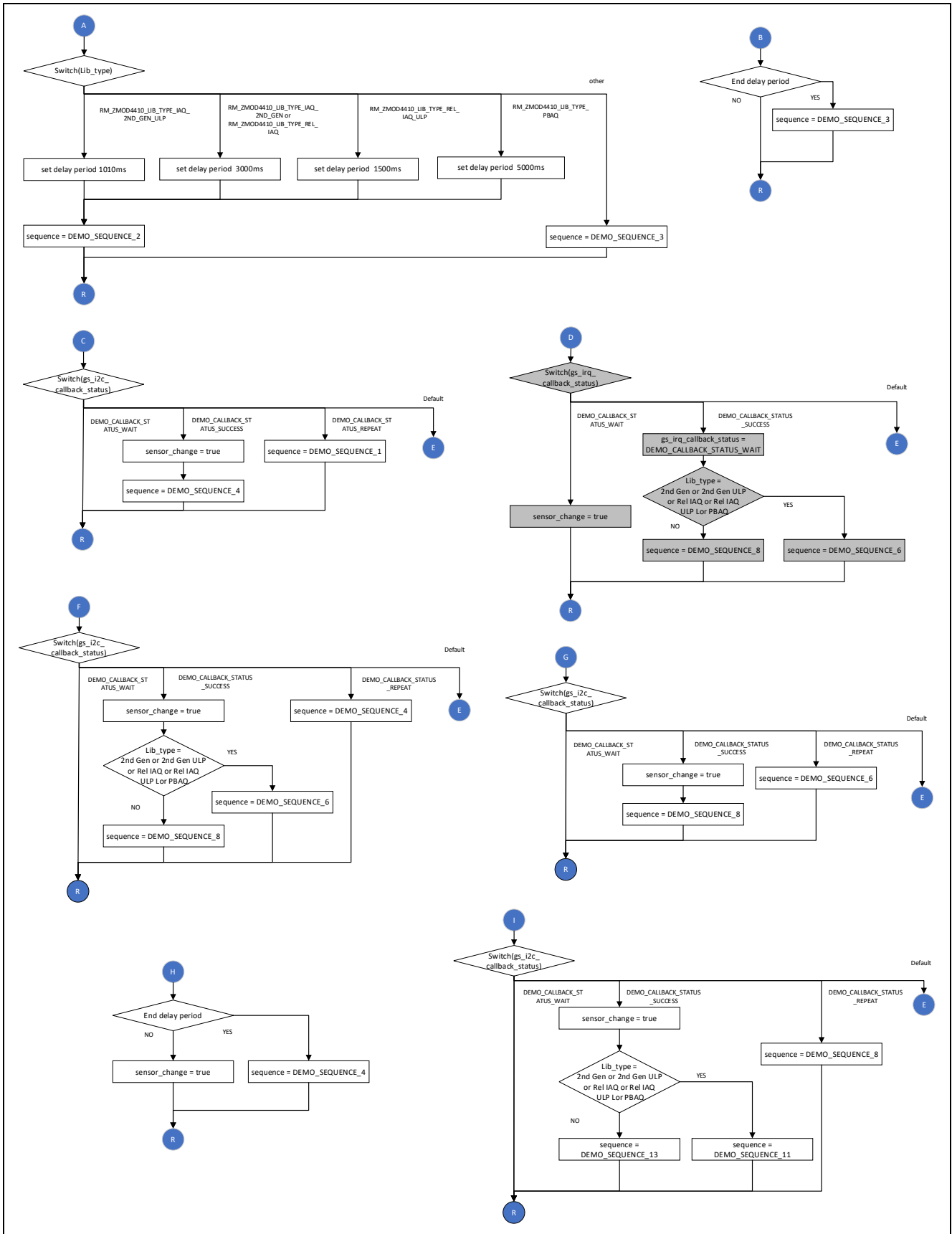
Figure 6-4 Flow 2 of ZMOD4410, ZMOD4450 Sample Software Main Processing
