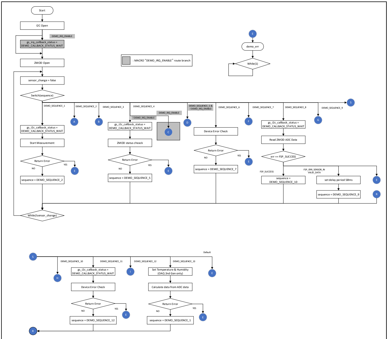
Figure 6-6 Flow 1 of ZMOD4510 Sample Software Main Processing
