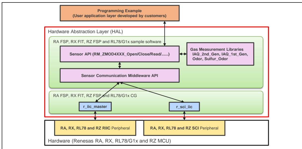
Figure 3-1 File Overview of ZMOD4410 Firmware
