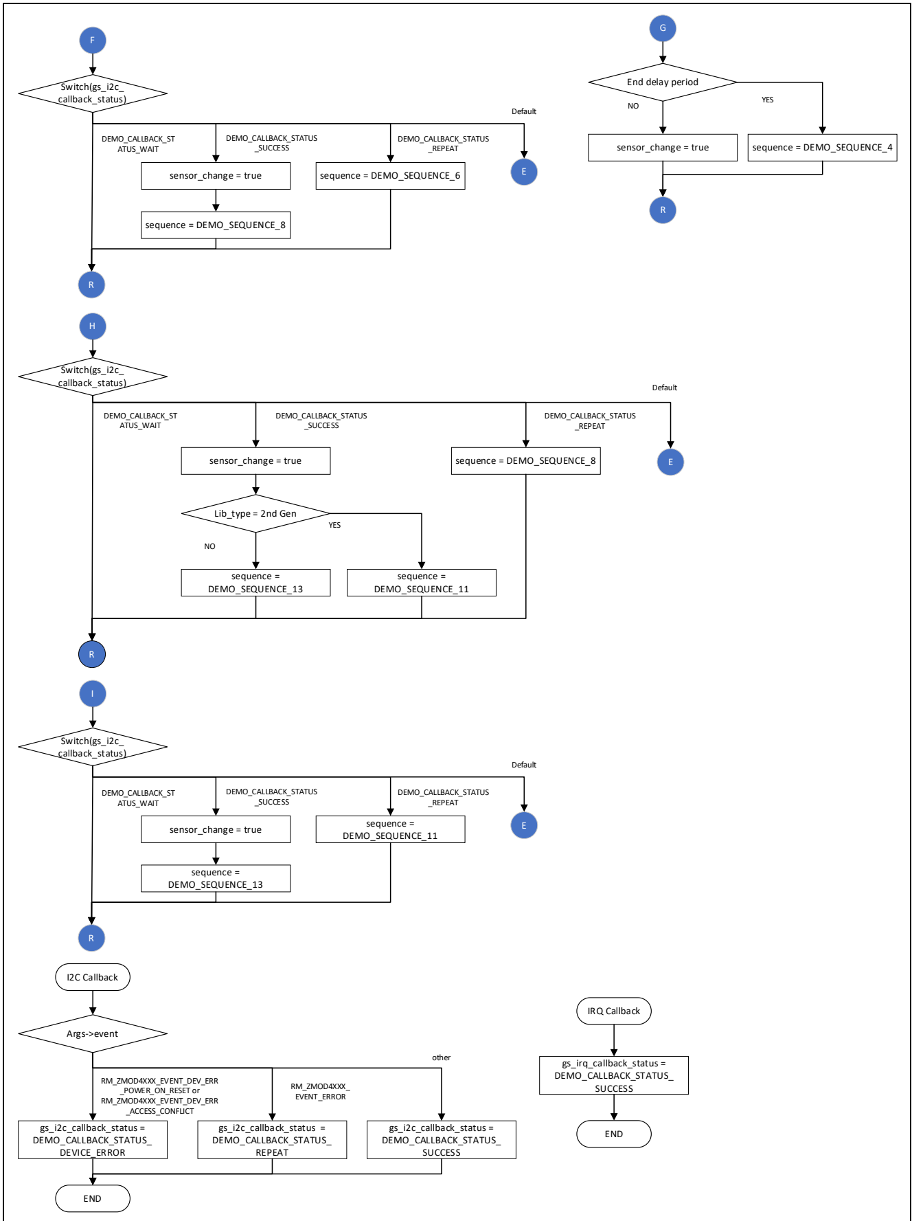
Figure 6-8 Flow 3 of ZMOD4510 Sample Software Main Processing
