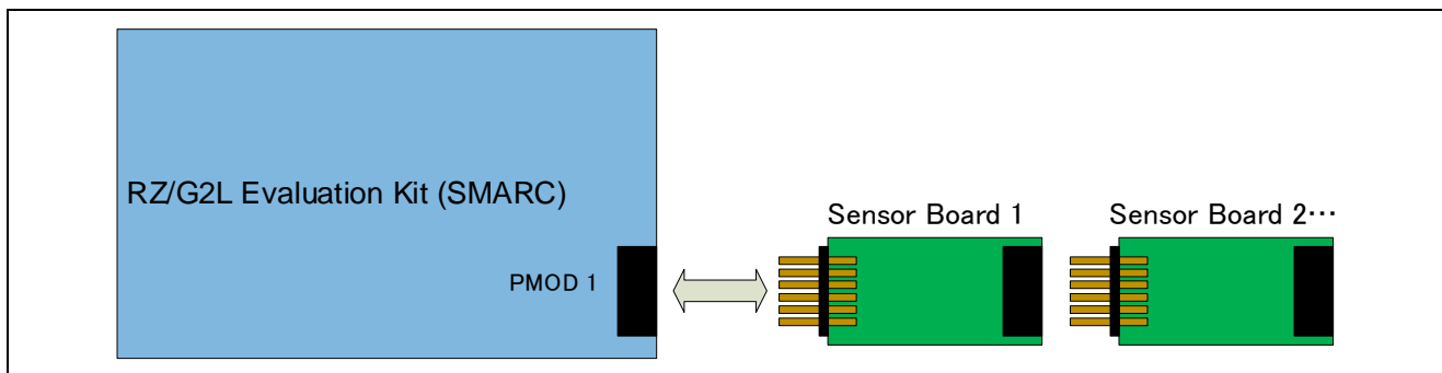
Figure 2-6 Hardware Connections for RZ Family
