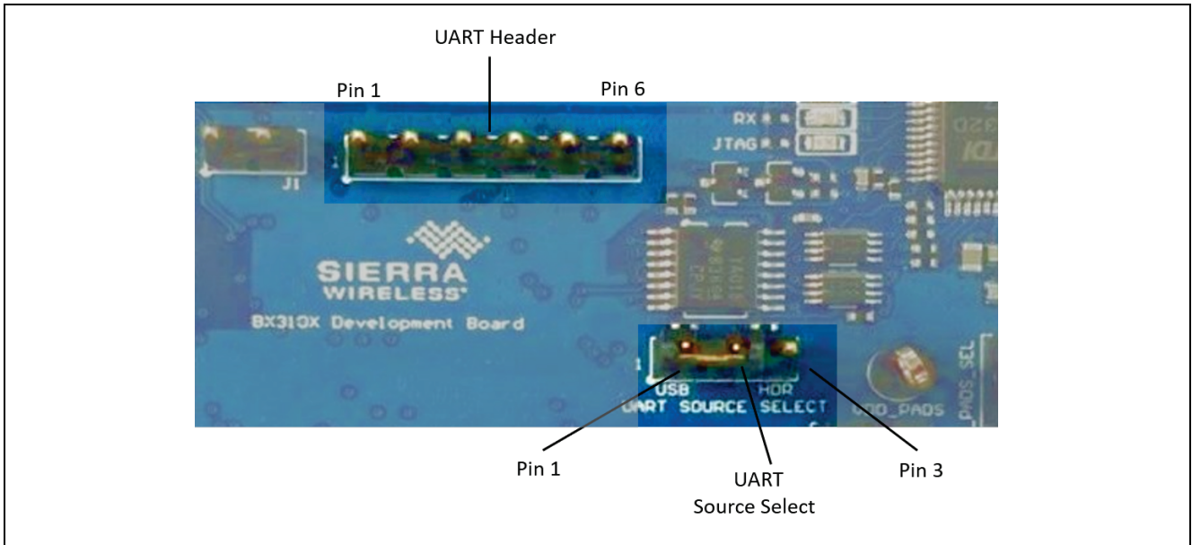
Figure 15. UART Header and UART Interface Selection
