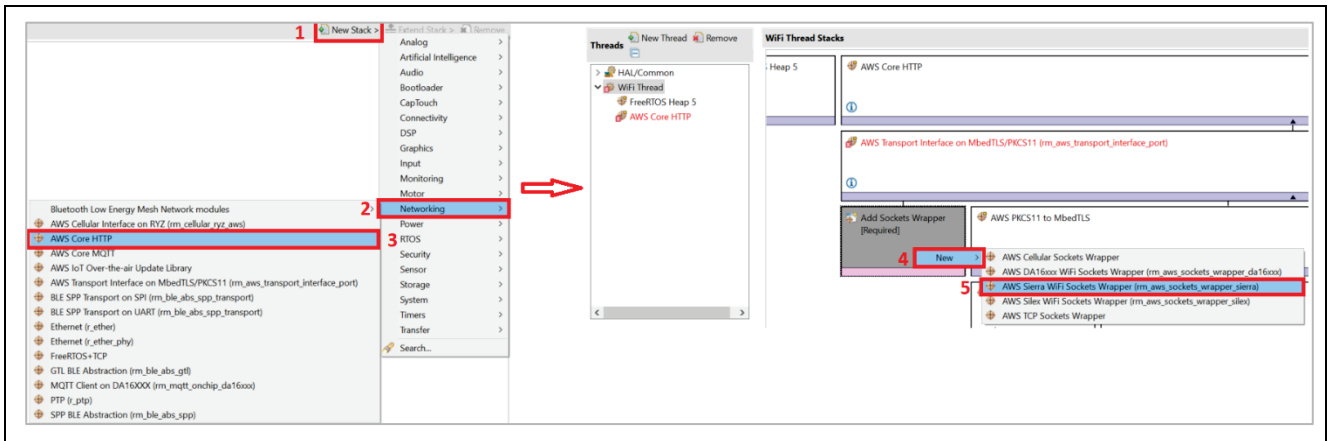
Figure 12. Adding Sierra Wi-Fi Module to the Project
