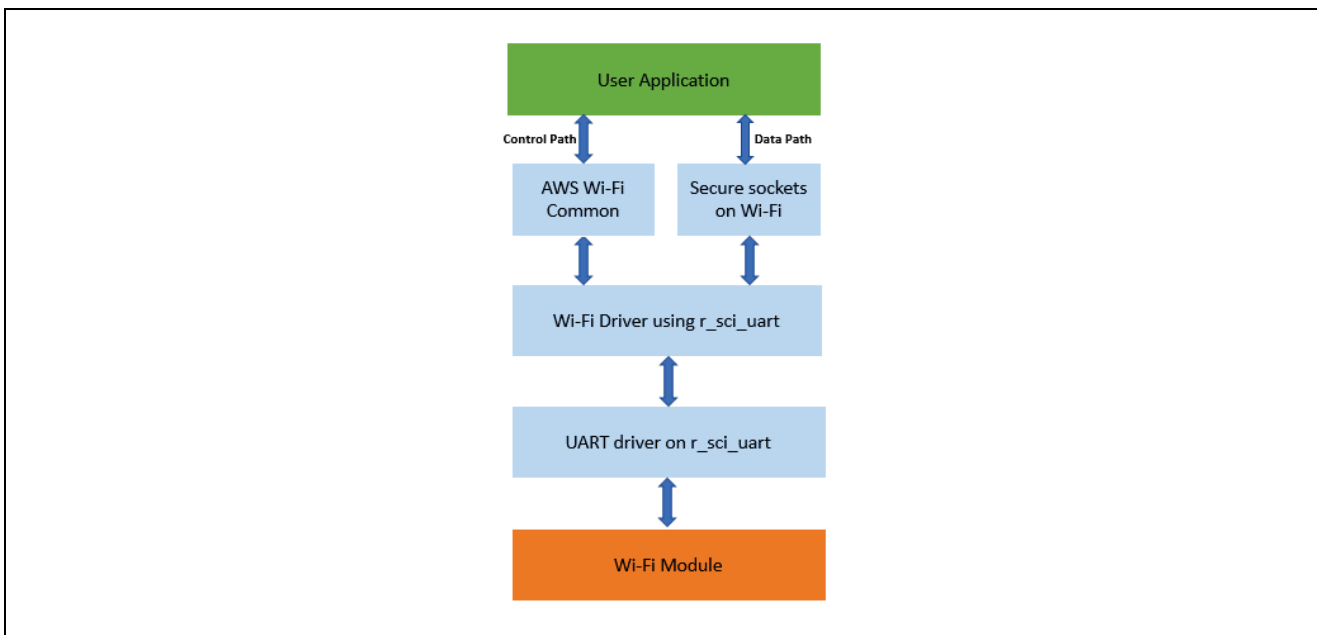
Figure 5. FSP Wi-Fi Driver Architecture
