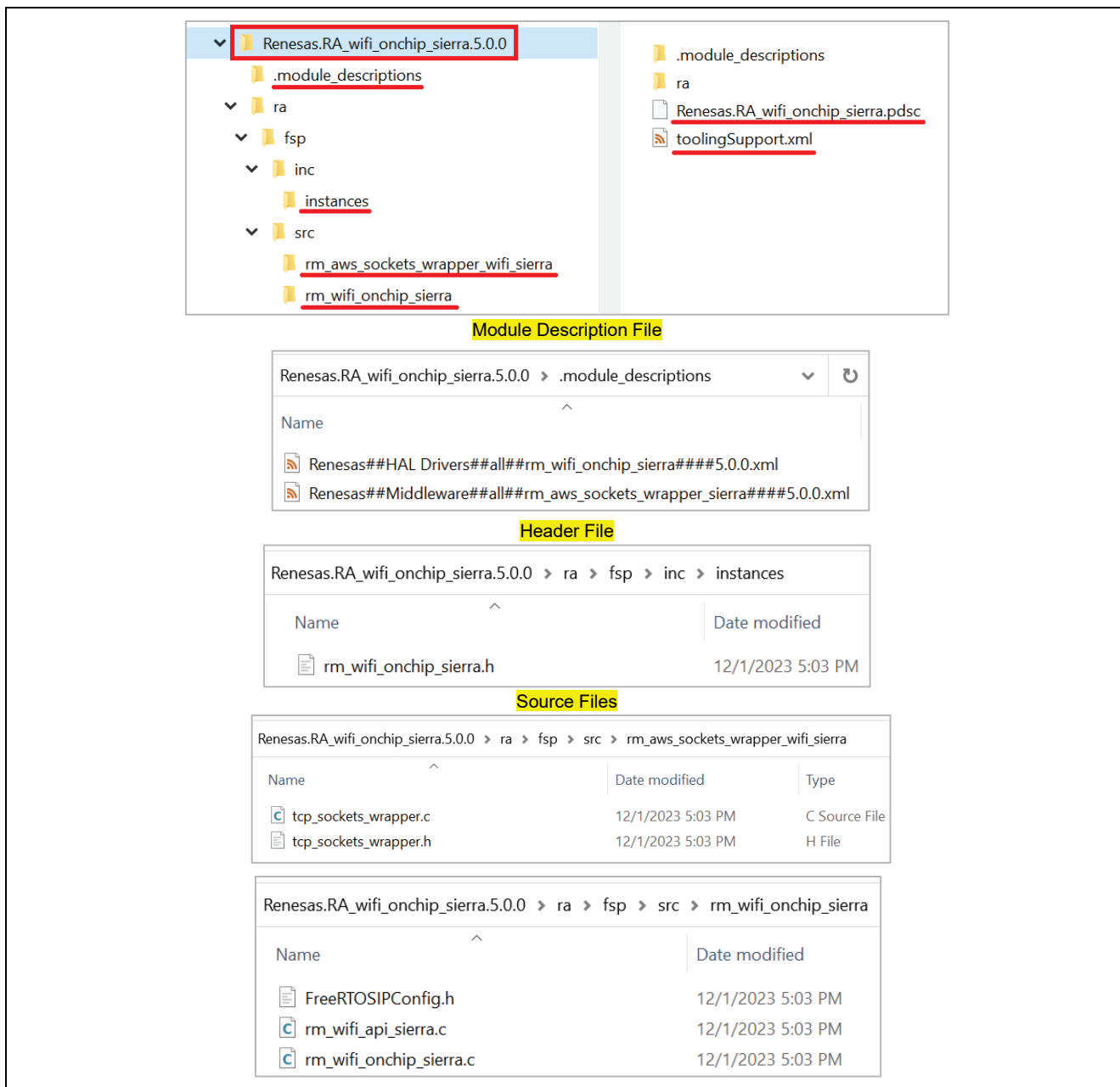
Figure 9. Folder Structure and File Information for the New Wi-Fi Driver Pack
