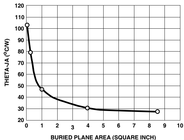
FIGURE 3. MLFP 7x7, 32 LEAD, THETA-JA vs BURIED PLANE AREA (1S2P-DA)
