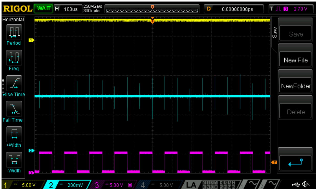
c) PWM signal is maximum
