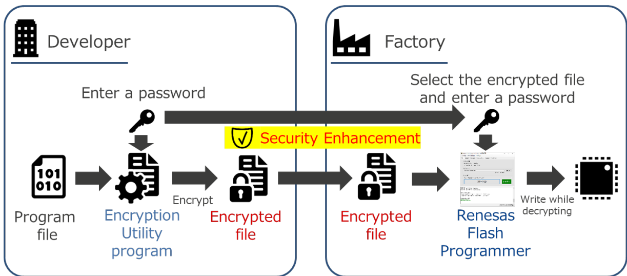
Figure 1 Encryption of program files
