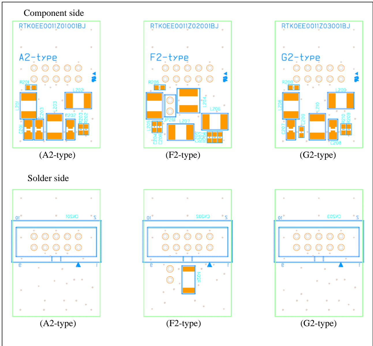
Figure 3-6 Filter board parts layout and silkscreen
