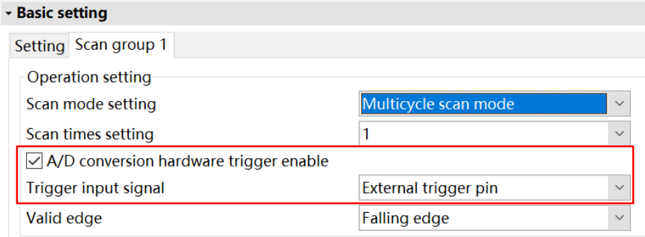
Figure 3-4. External trigger pin setting
