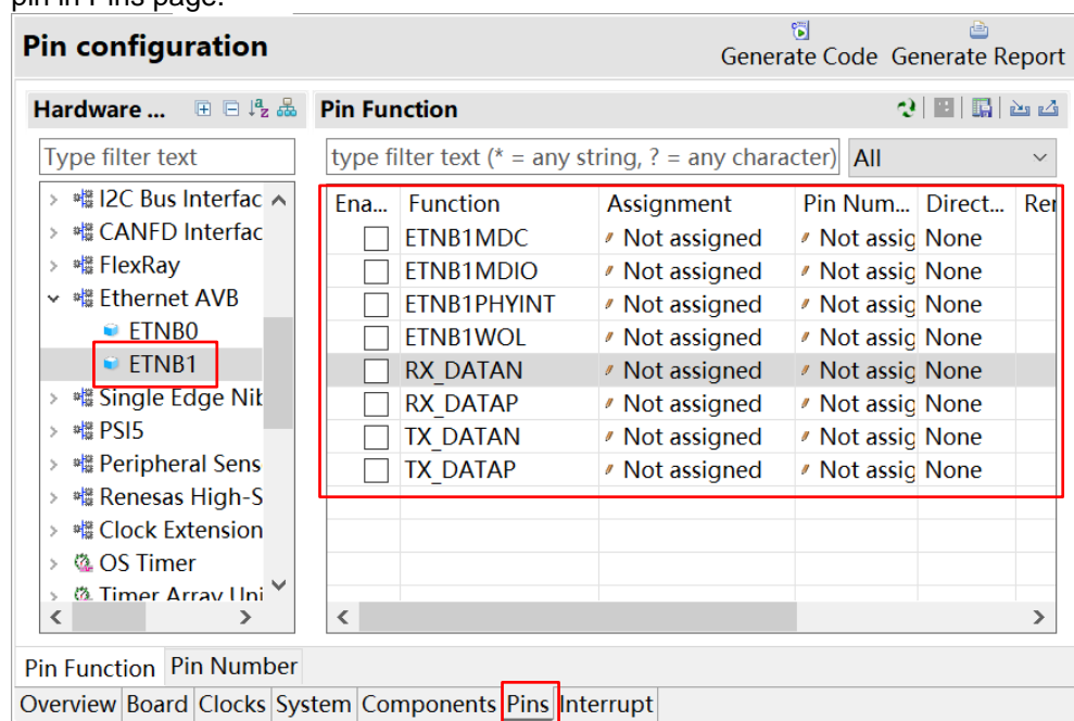
Figure 3-6. ENTB1 is supported in Pins page
