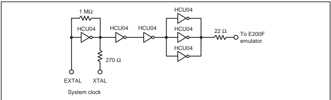
Figure 8 Clock Oscillator
