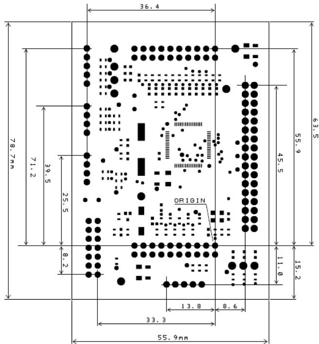
[Unit: mm] Component side View
