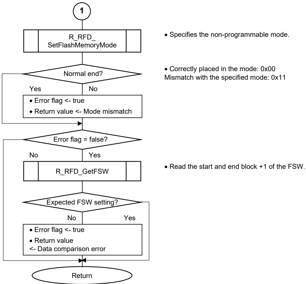
Figure 5-12 Flowchart of Sample Processing for Controlling Extra Area (FSW) Reprogramming (2/2)
