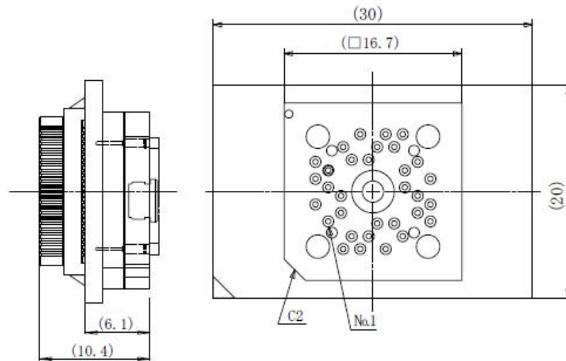
< Bottom view >
