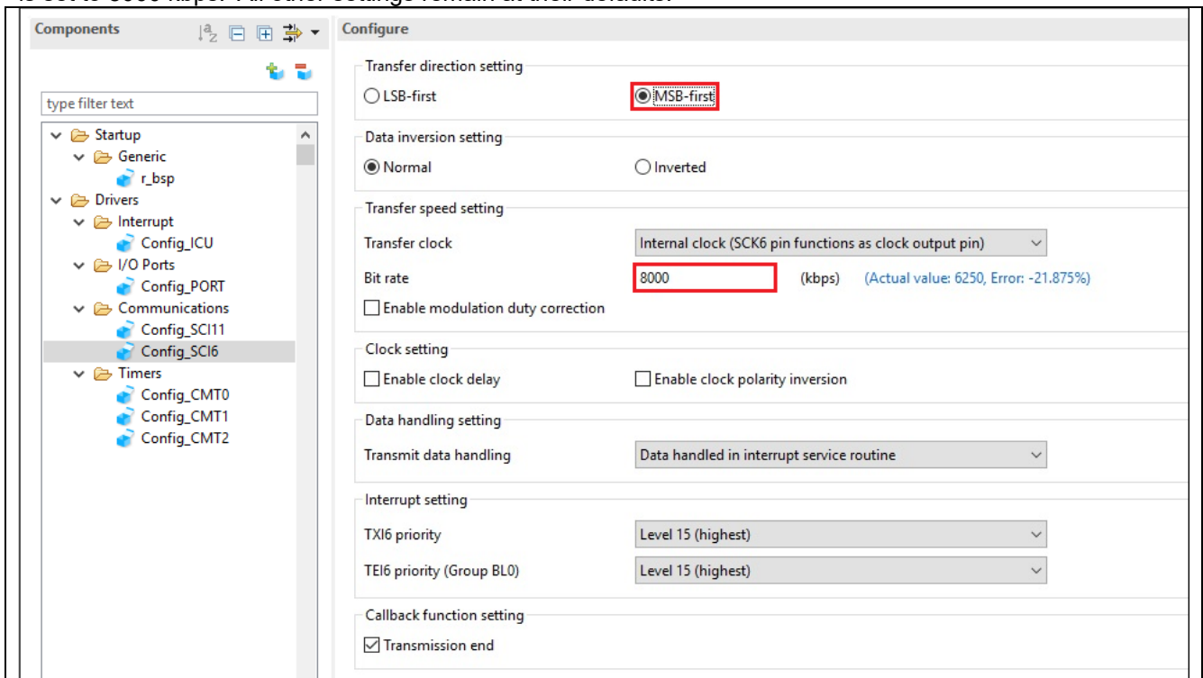
Figure 4-36 Config_SCI6 setting
