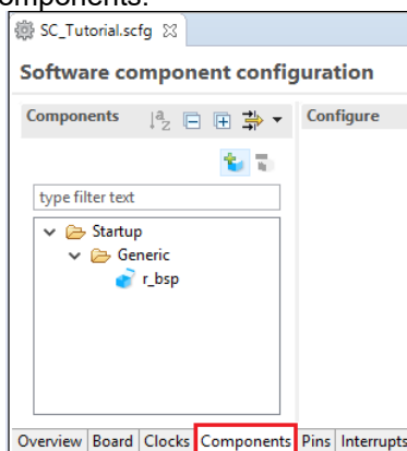
Figure 4-6 Component page
