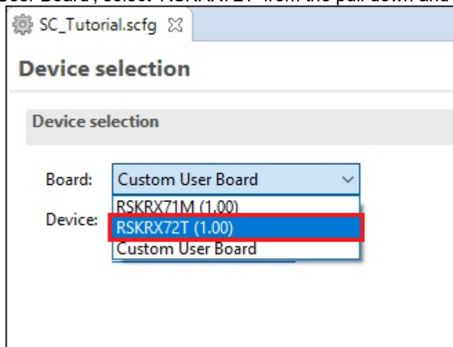
Figure 4-3 Select board
