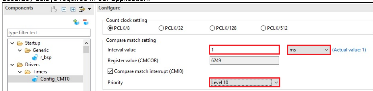
Figure 4-11 Config_CMT0 setting
