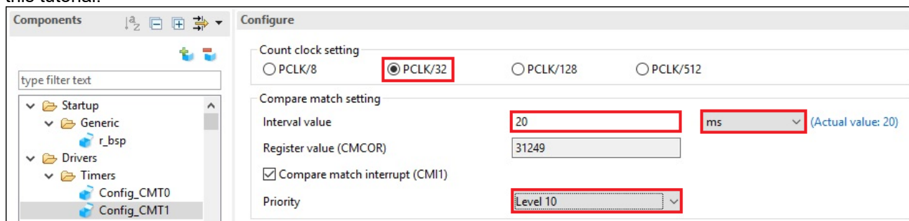
Figure 4-13 Config_CMT1 setting
