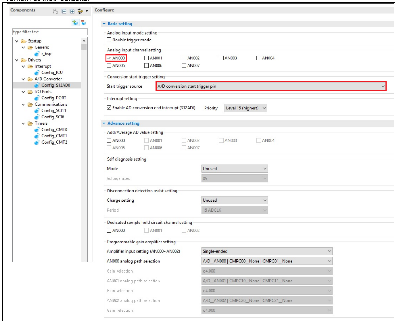
Figure 4-39 Config_S12AD0 setting (1)
