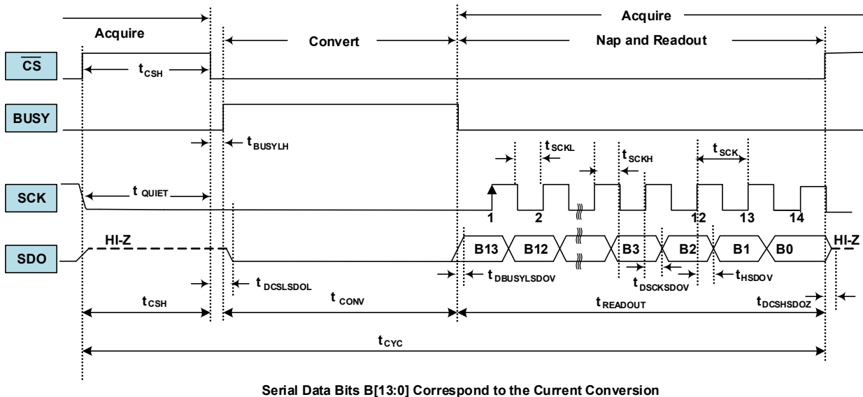
Serial Data Bits B[13:0] Correspond to the Current Conversion
