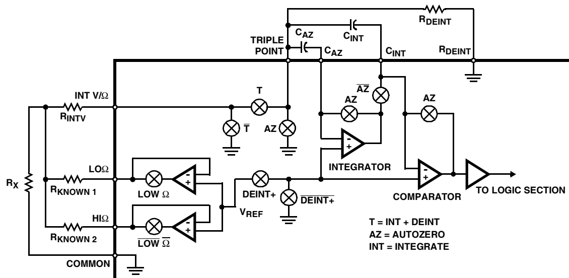
FIGURE 7. DETAILED CIRCUIT DIAGRAM FOR RATIOMETRIC \Omega MEASUREMENT
