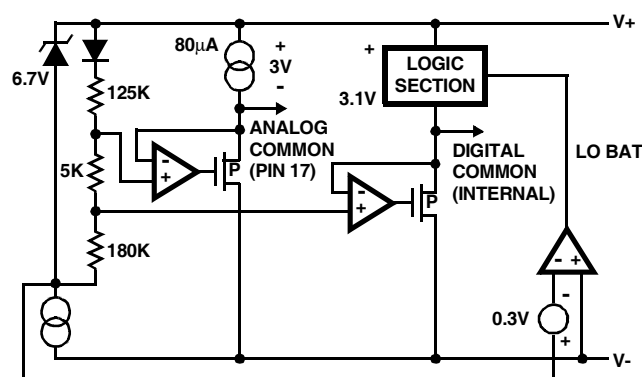
FIGURE 9. ANALOG AND DIGITAL COMMON VOLTAGE GENERATOR CIRCUIT
