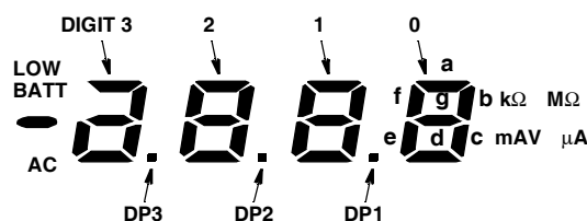
FIGURE 2. DISPLAY SEGMENT NOMENCLATURE
