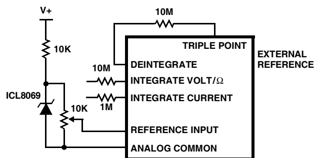
FIGURE 12. EXTERNAL VOLTAGE REFERENCE CONNECTION
