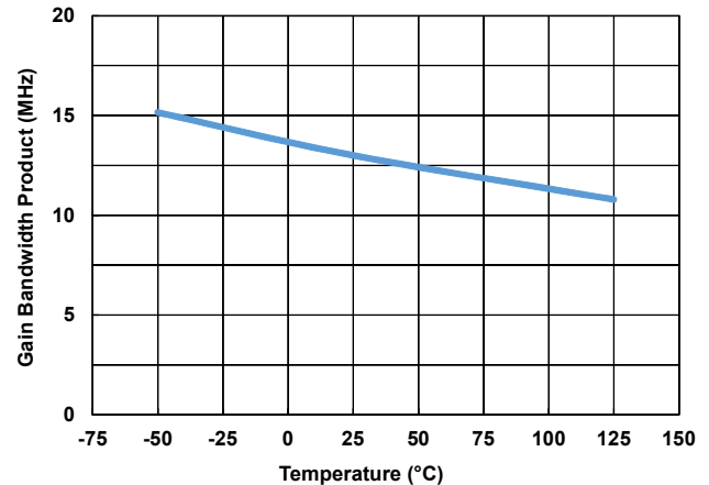
Figure 30. Error Amplifier GBWP vs Temperature
