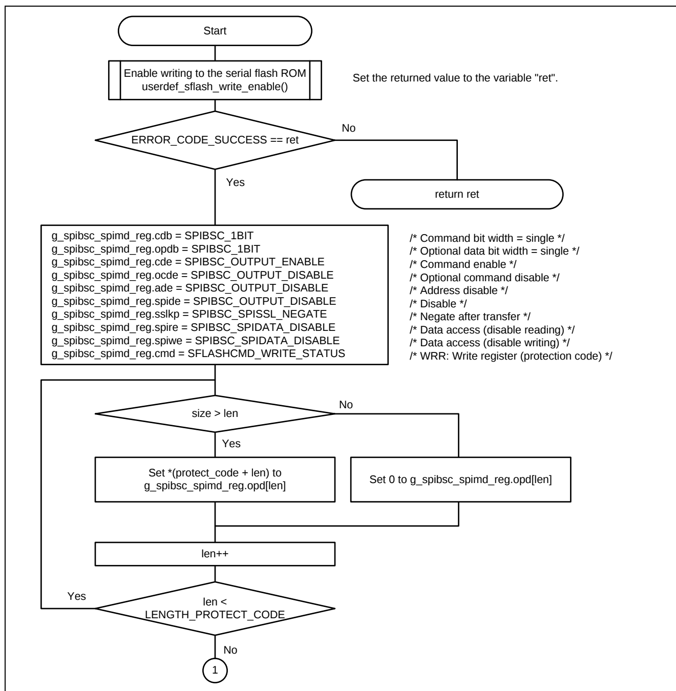
Figure 5.13 spibsc_set_protect_code Function Processing (1/2)
