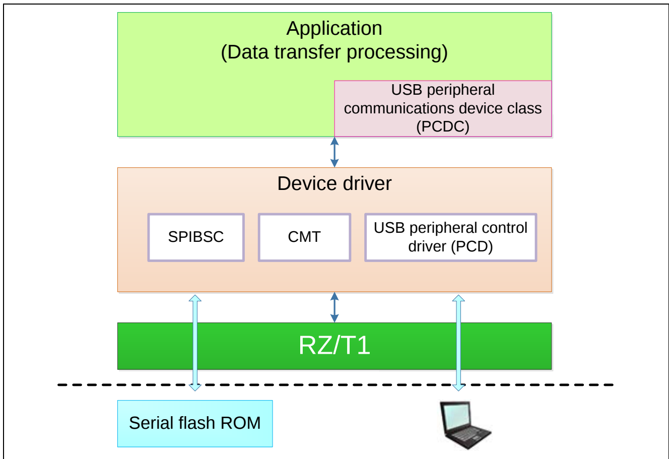
Figure 5.5 Software Configuration
