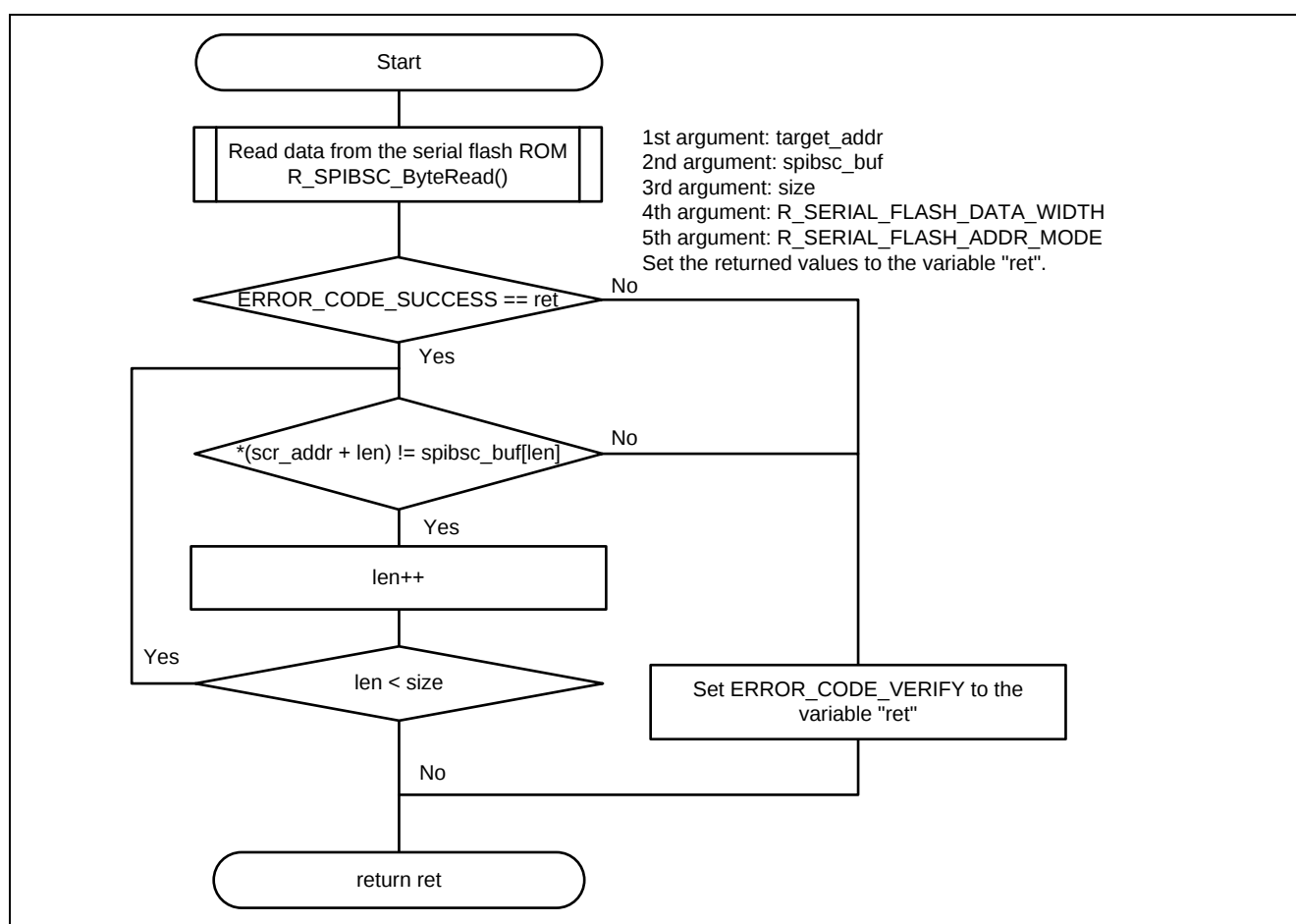
Figure 5.14 spibsc_verify_data Function Processing
