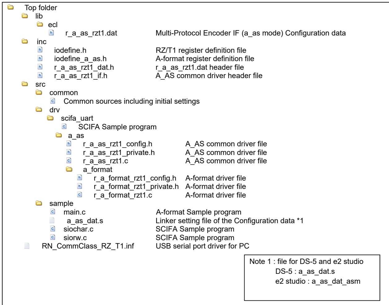
Figure 2.1 File Structure
