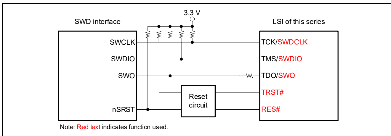
Figure 6.3 Example of SWD interface connection
