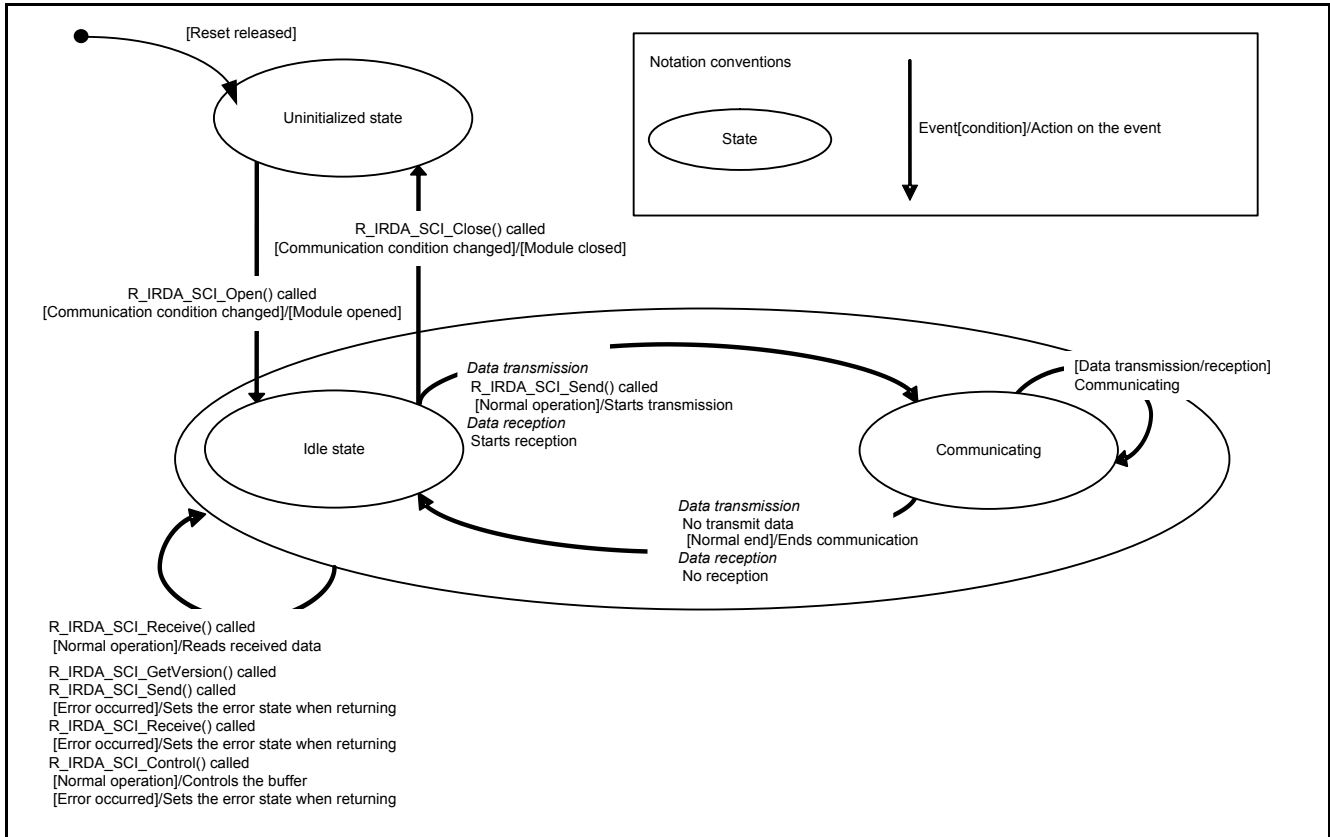
Figure 1.1 State Transitions in the IrDA FIT Module
