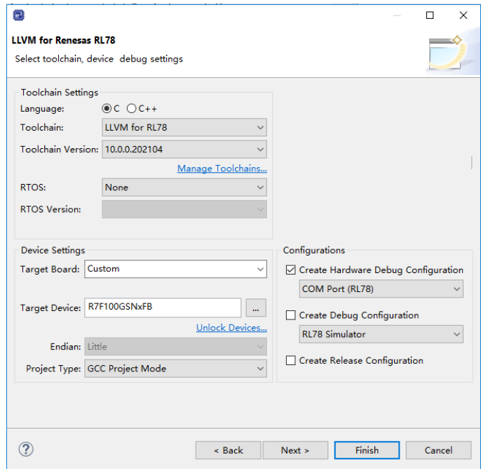
LLVM for Renesas RL78 C/C++ Executable Project
