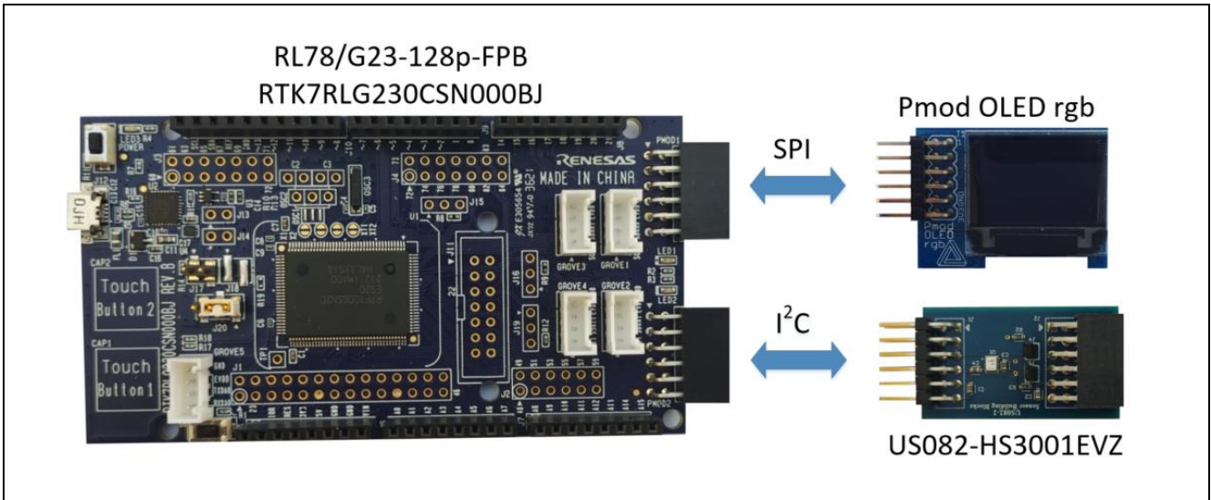
Figure 3.1 System Composition
