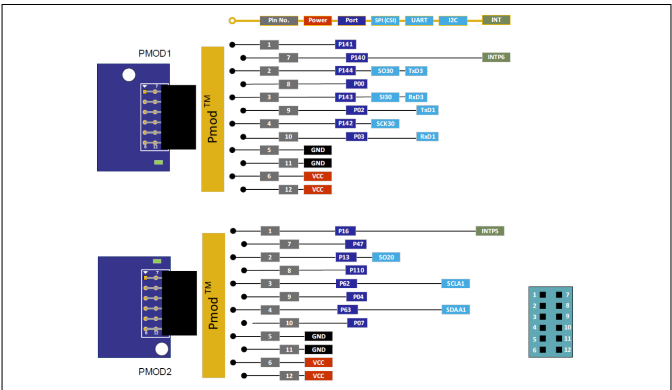
Figure 3.2 RL78/G23-128p-FPB PMOD Interface
