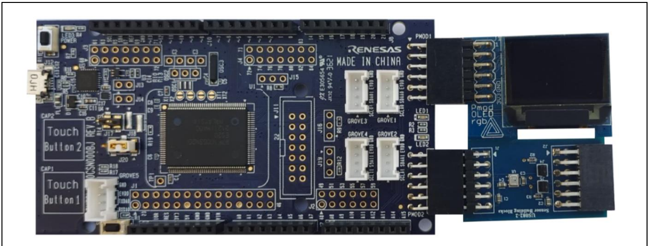
Figure 4.1 Hardware Composition
