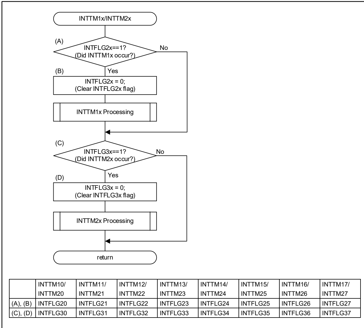
図 1-9 INTTM1x/INTTM2x Interrupt Judgement Example
