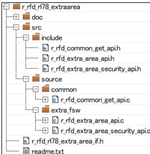
The developed r_rfd_rl78_extraarea folder
