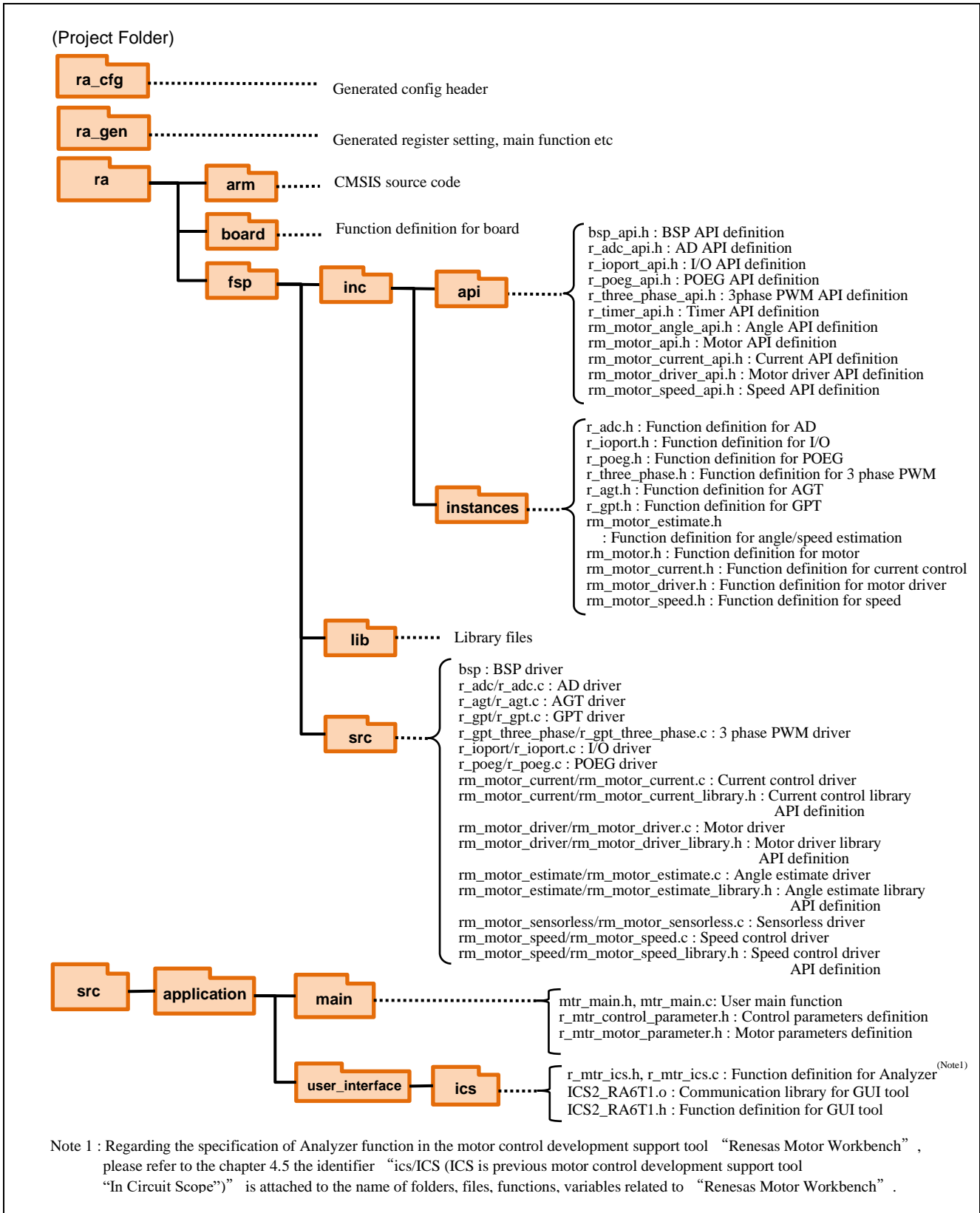
Figure 2-6 Folder and file configuration
