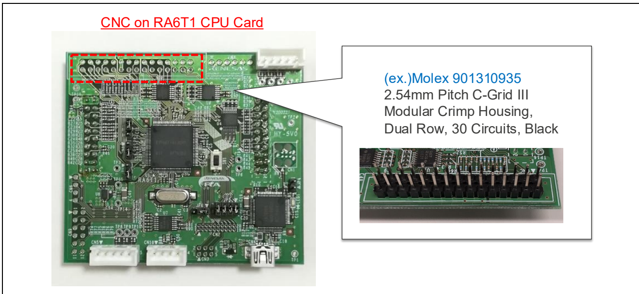
Figure 2-6 Mounting the pin header to the CPU card
