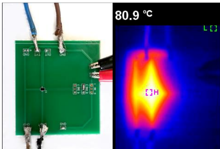
Figure 7. Visible (left) and Thermal (Right) Images of the SLG59H1302C in a 5 mm 2 , 28-Lead WLCSP Mounted on a Type-A PCB. T_A = 25\text{ }^{\circ}\text{C} , V_{BUS} = 5\text{ V} , I_{LOAD} = 4\text{ A} .
