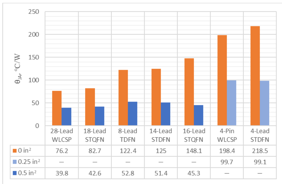
Figure 33. Thermal Resistance vs. Package Type and Polygon Area
