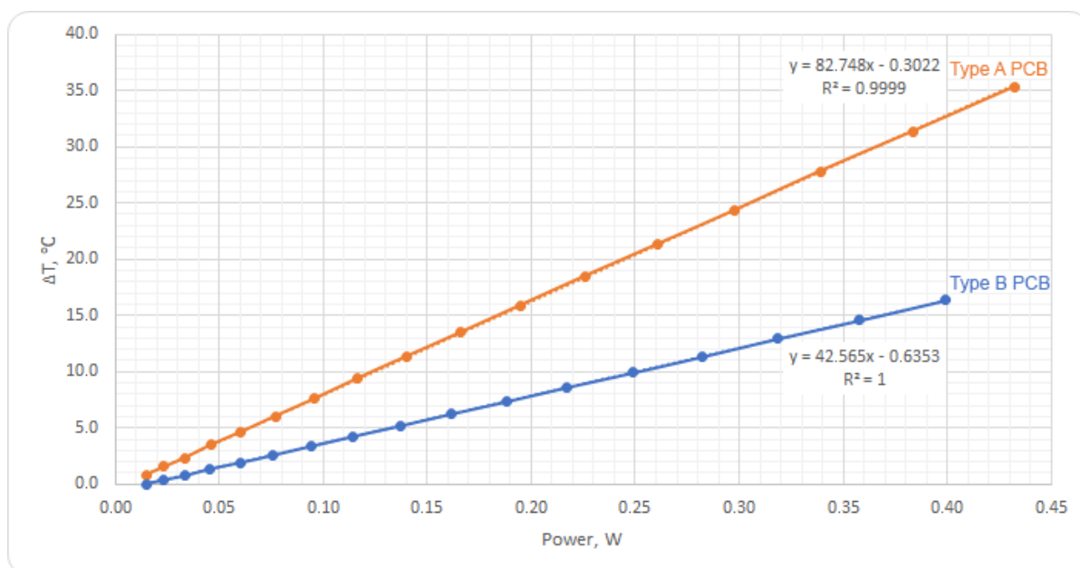
Figure 10. Package Power Dissipation vs. Temperature Difference for the SLG59H1006V in a 4.8 \text{ mm}^2 , 18-Lead STQFN Package
