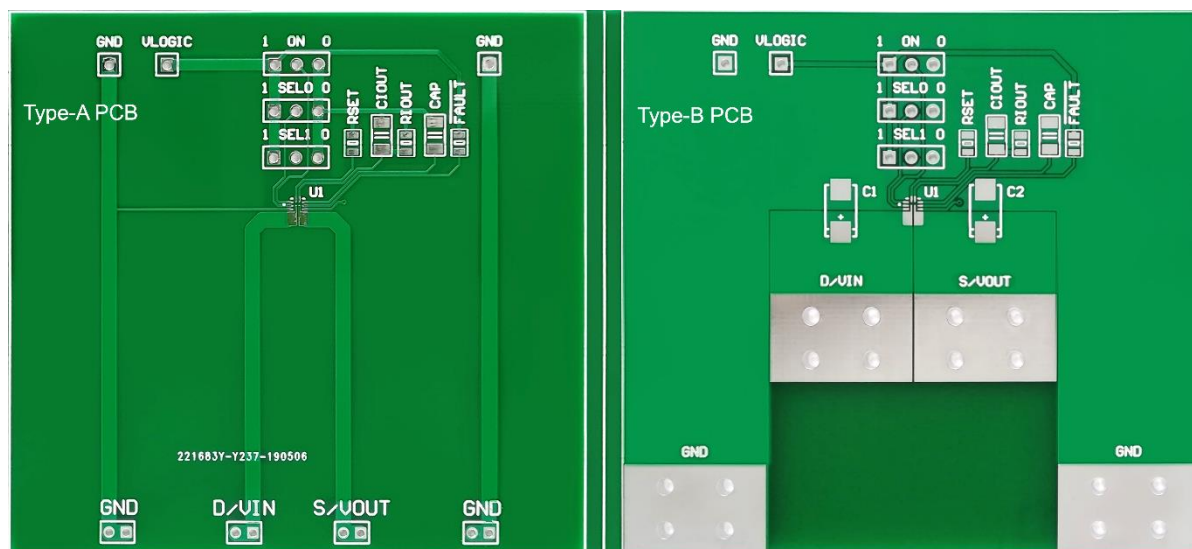
Figure 9. Type-A (left) and Type-B (right) PCB Evaluation Boards for \theta_{JA} Measurements of the SLG59H1006V in a 4.8 \text{ mm}^2 , 18-Lead STQFN Package
