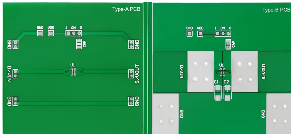
Figure 17. Type-A (left) and Type-B (right) PCB Evaluation Boards for \theta_{JA} Measurements of the SLG59M1568V in a 3 mm 2 , 14-Lead STDFN Package
