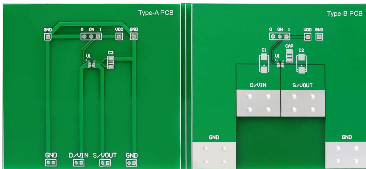
Figure 13. Type-A (left) and Type-B (right) PCB Evaluation Boards for \theta_{JA} Measurements of the SLG59M301V in a 3 mm 2 , 8-Lead TDFN Package
