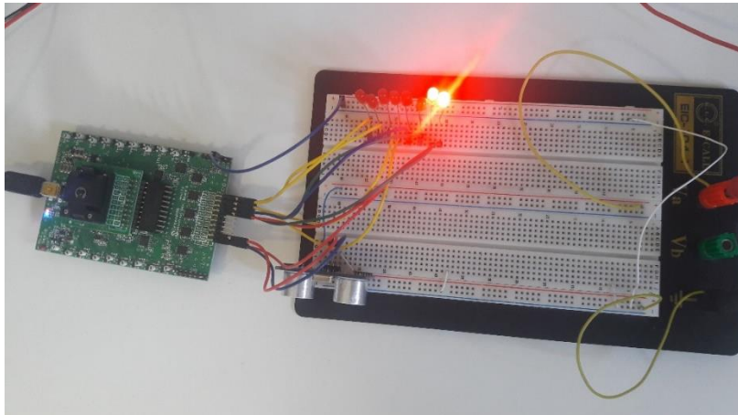
Figure 15: Circuit Test Measuring Distance D Within the Range 2: 150\text{ cm} < D < 175\text{ cm}
