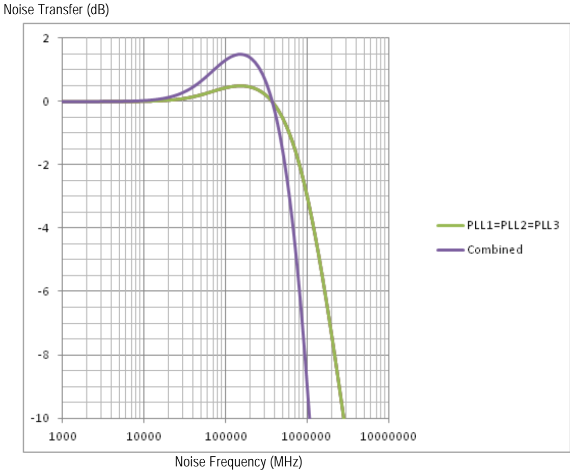
Figure 3. Cascading 3 PLLs, each with 0.5dB Jitter Peaking
