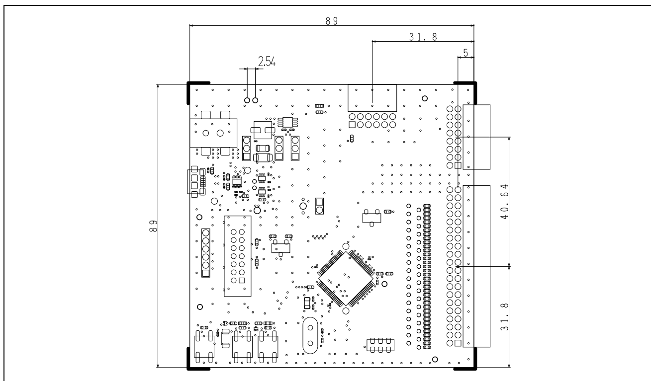
Figure 2-3. Board Dimensions
