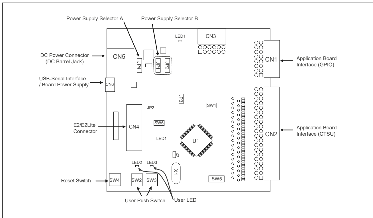
Figure 2-2. Parts Location
