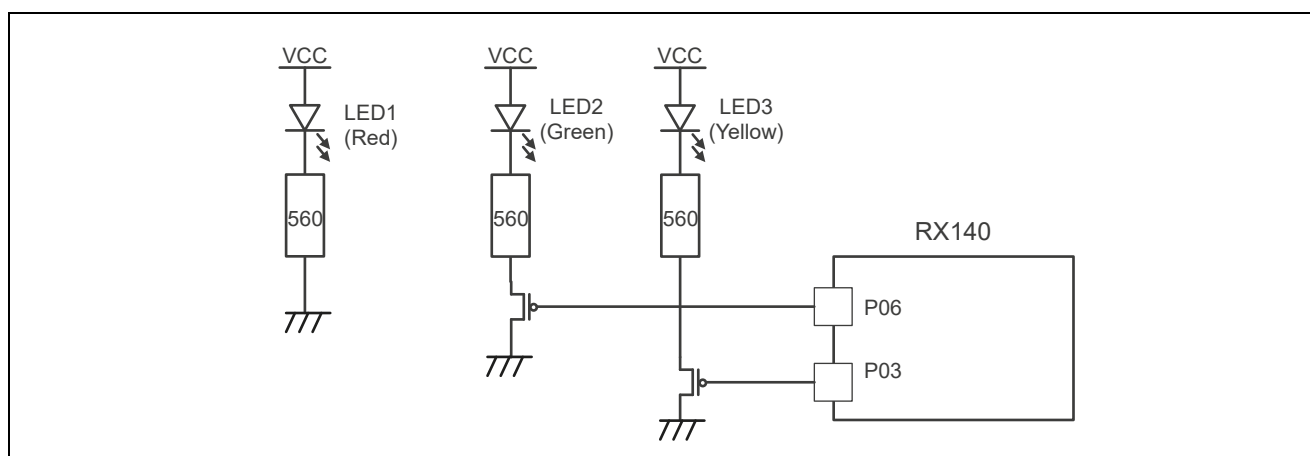
Figure 2-9. LED Circuit
