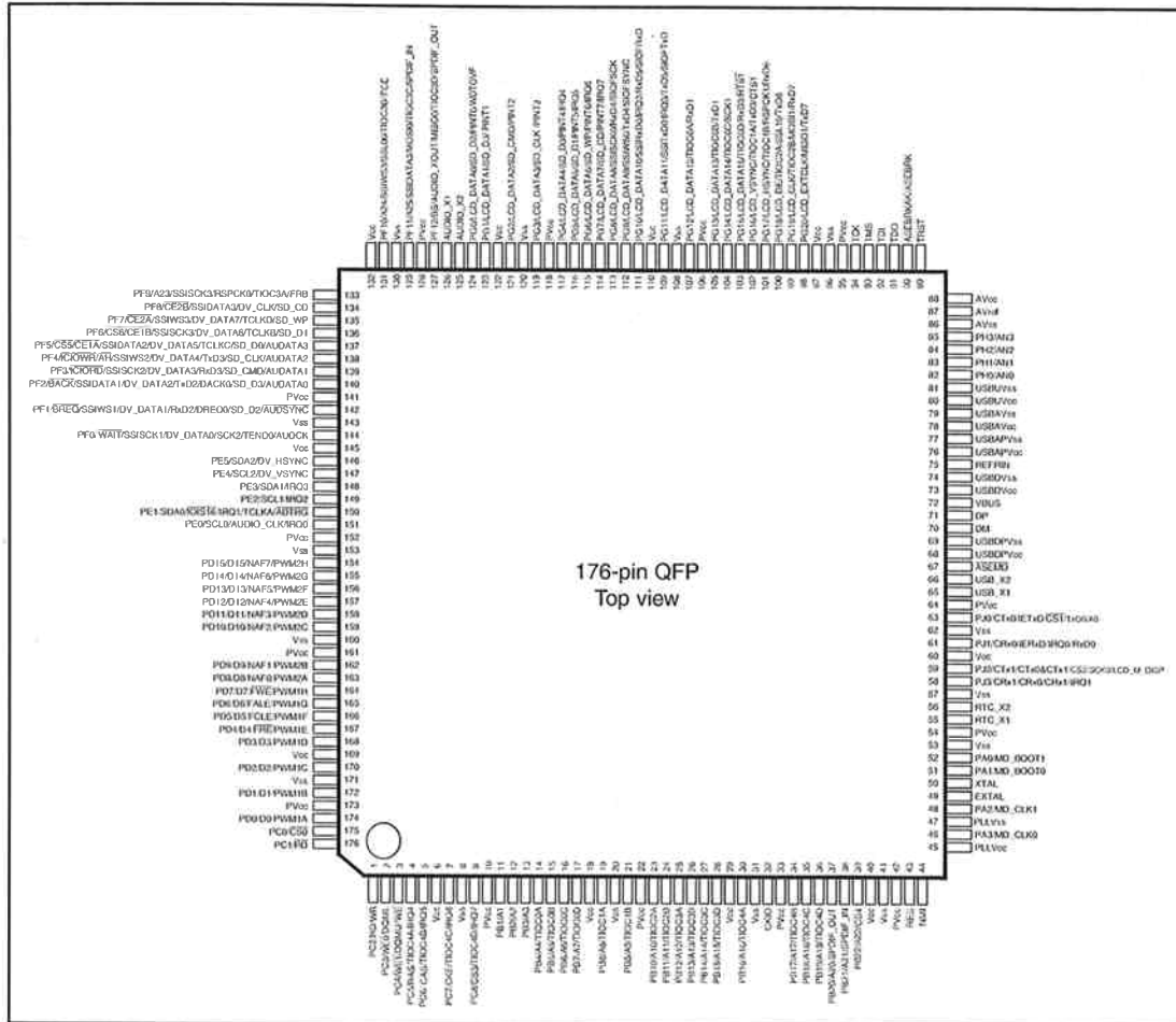
Figure 1.2 (1) Pin Assignment for the SH7262 Group
