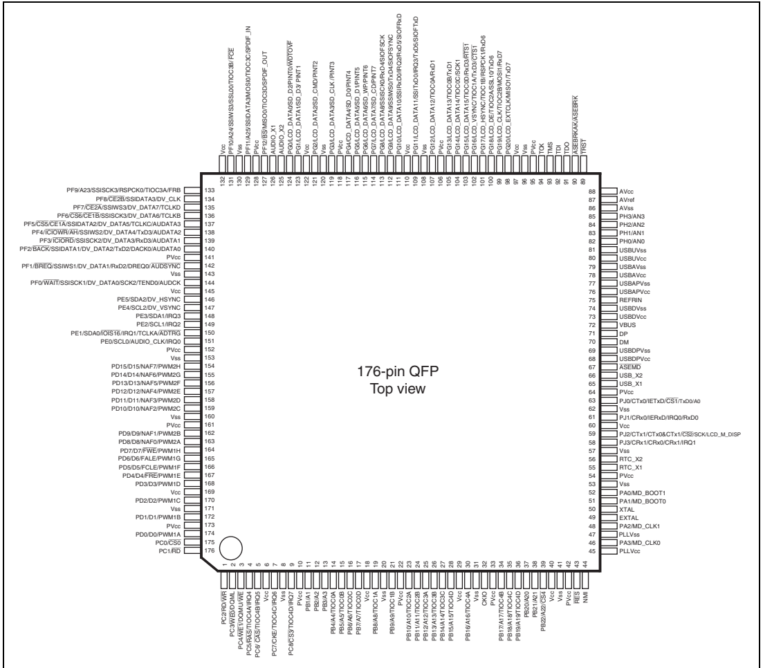
Figure 1.2 Pin Assignment
